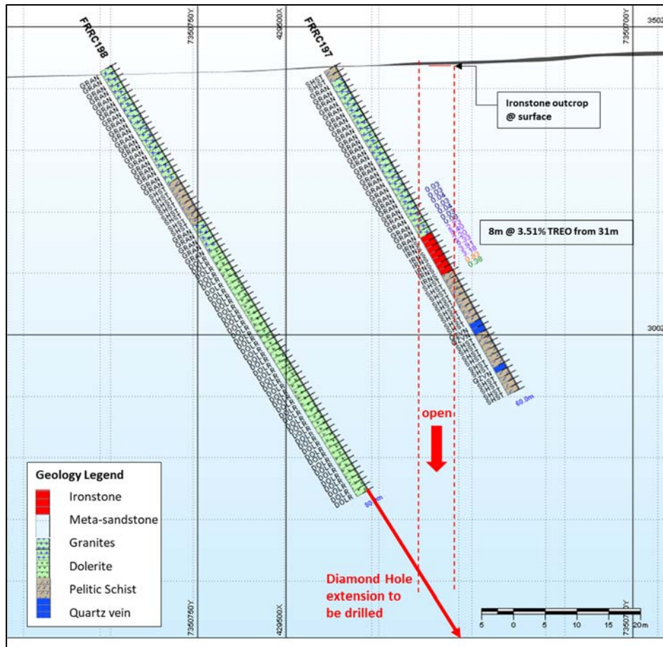
Fig 4. Section B-B', Cross-section (see plan) looking south east through Fraser's South mineralisation.
