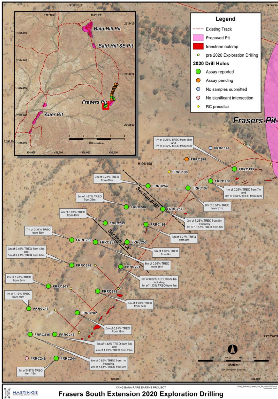
Fig 2. Exploration Drilling results from Fraser's South and results received.
