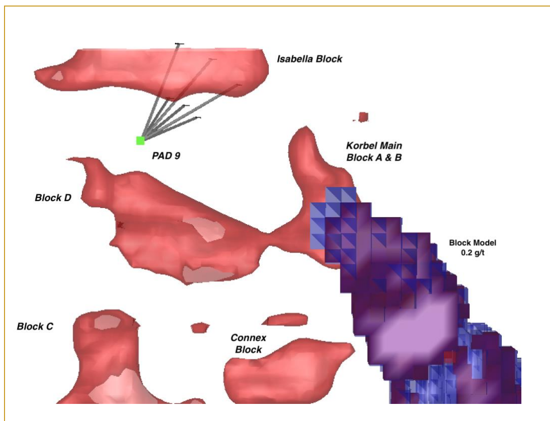
Figure 2. Isabella Drill hole layout with 3D IP Chargeability Anomalies (15 mV/V) and Block Model
