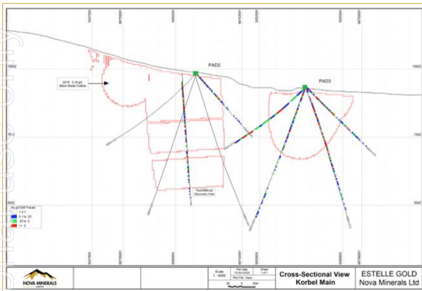
Figure 4. Cross Section View of Korbelt Main
