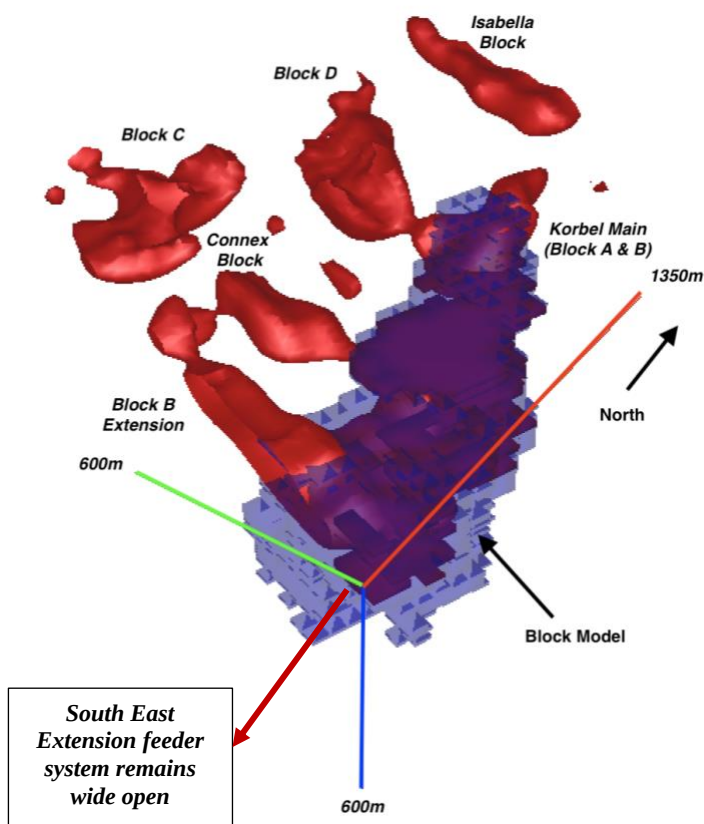
Figure 1. Korbel Isabella Block, 3D model showing IP Chargeability anomalies (15mV/V) and target zones.
