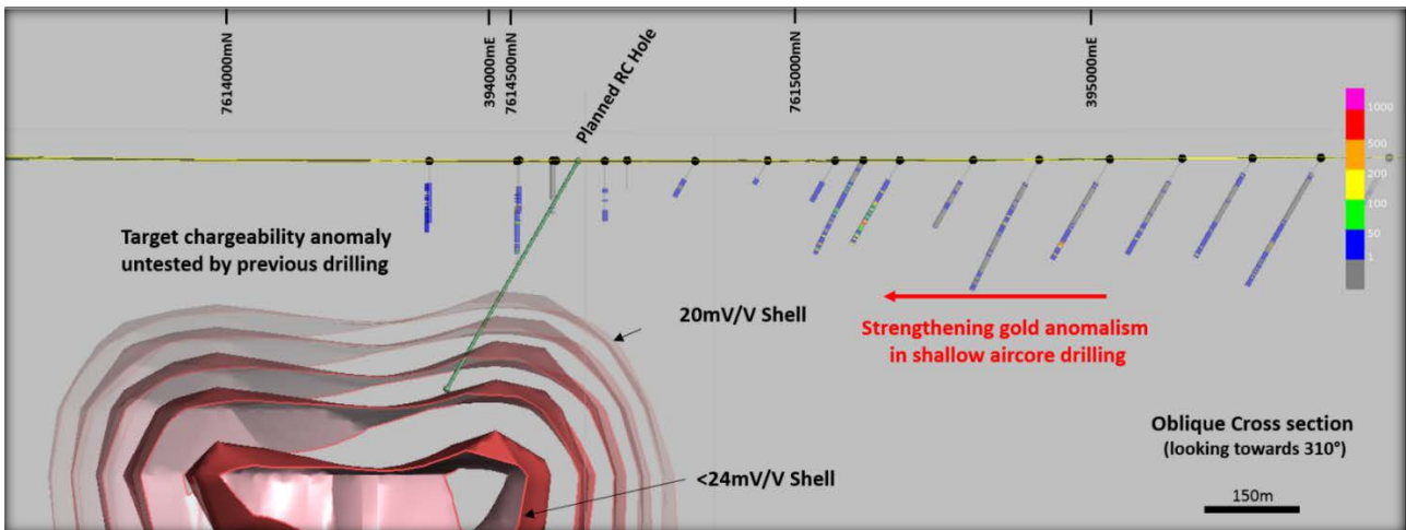
Figure 4 – Elsa Prospect - Section of 3D chargeable isosurfaces and planned RC drill hole location
