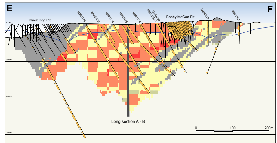
Cross section E - F
