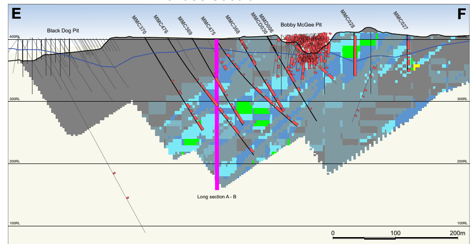
Cross section E - F
