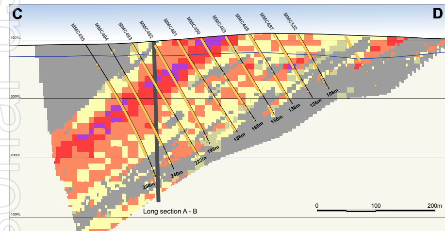
Cross section C - D
