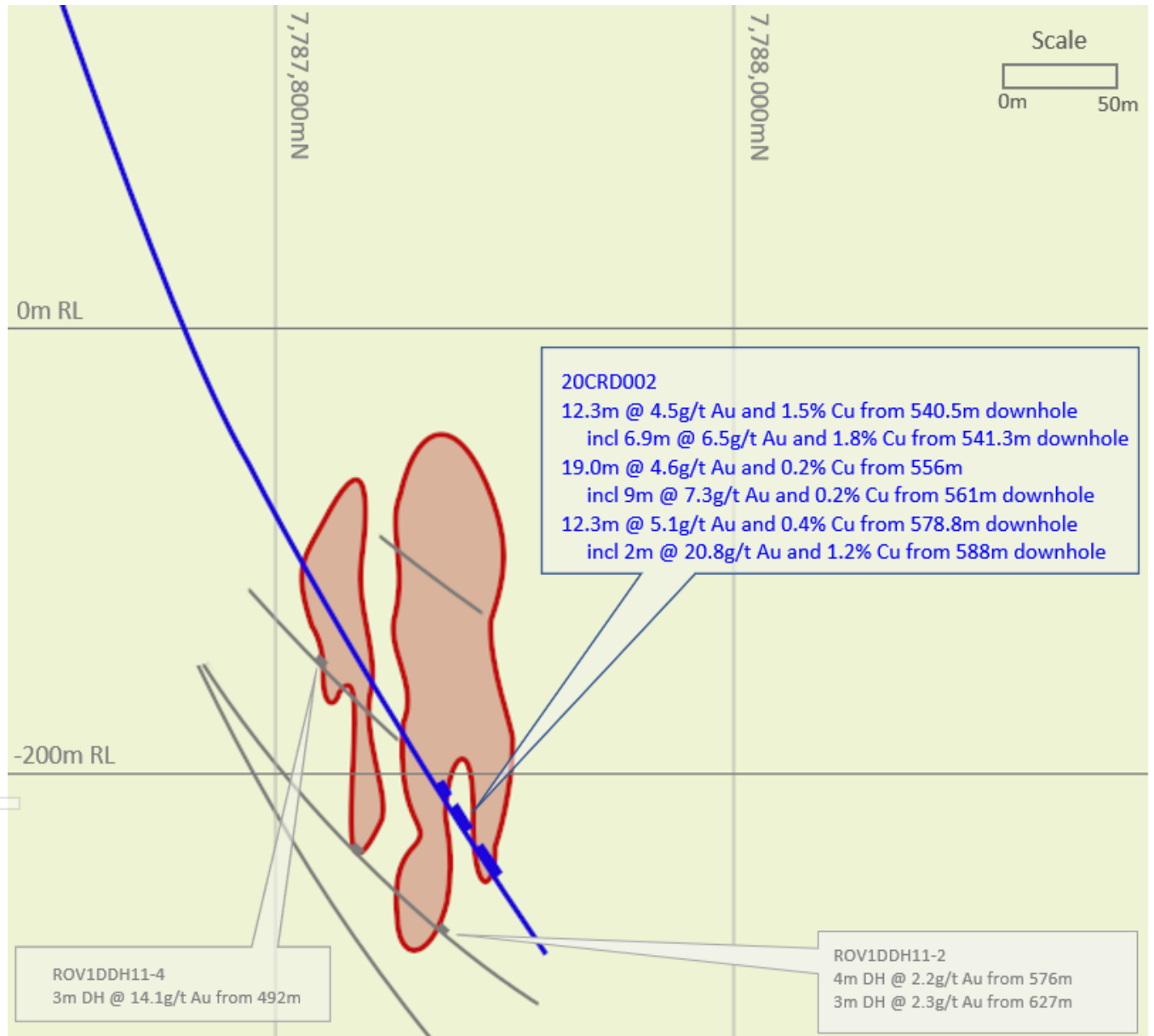
Figure 1: Cross section of Hole 20CRD002
