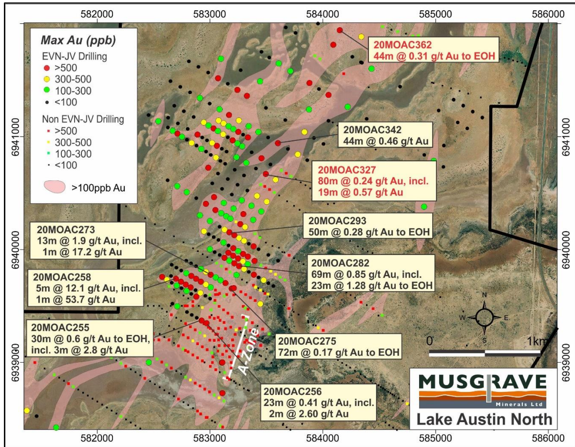
Figure 3: Location plan showing 2020 EVN JV aircore drill hole locations at Lake Austin North and includes historical drill holes. Maximum gold in hole is presented on the gradational colour scheme
