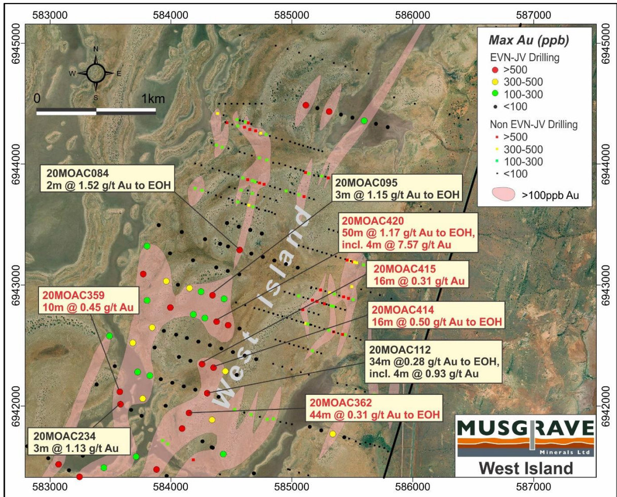
Figure 2: Location plan showing 2020 EVN JV aircore drill hole locations at West Island and includes historical drill holes. Maximum gold in hole is presented on the gradational colour scheme
