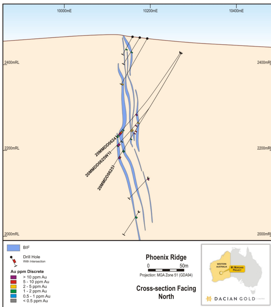
Figure 8: 20m cross section at 12880mN of the stratigraphic interpretation model for Phoenix Ridge
