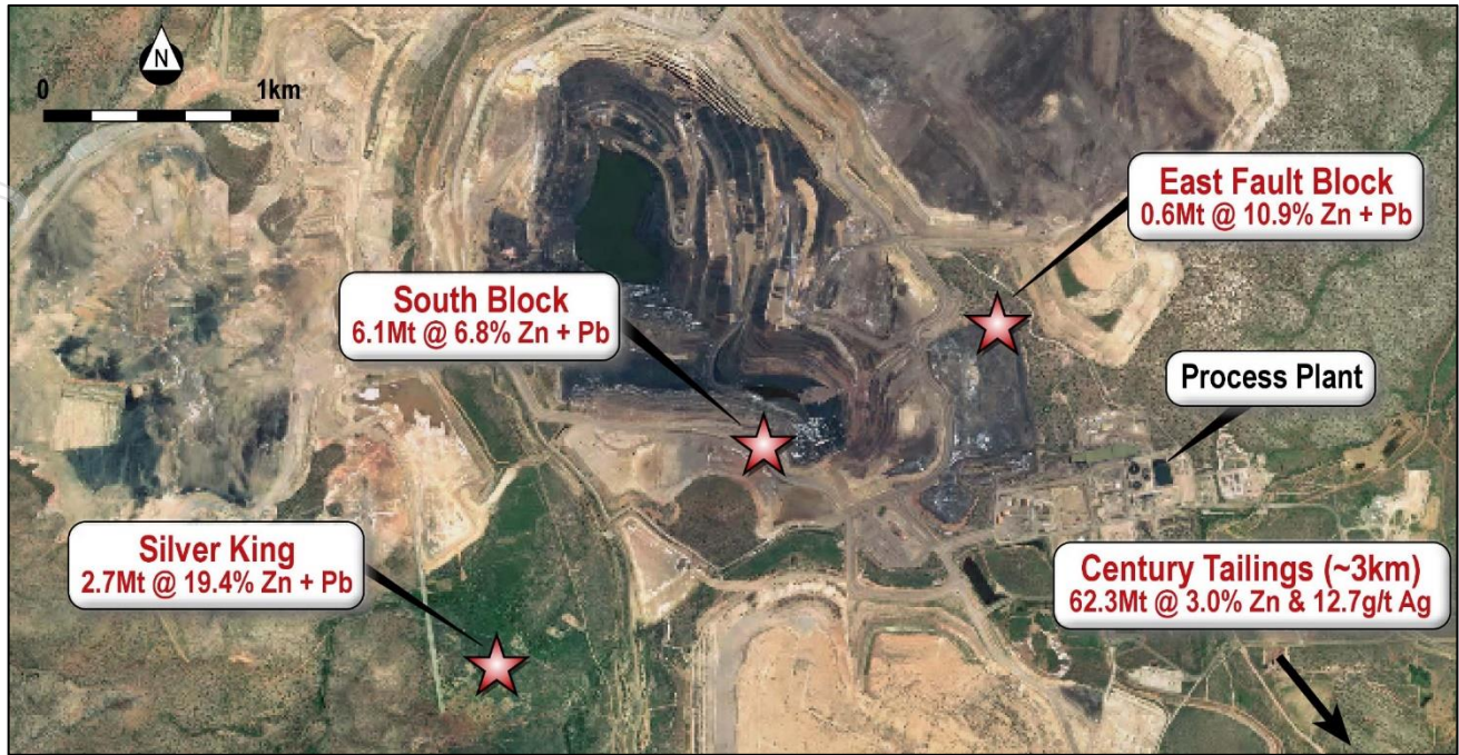
Figure 4: Location of Silver King and other existing Mineral Resources and Ore Reserves on the Century Mining Lease
