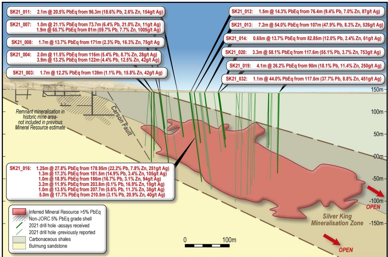
Figure 1: Silver King long section showing highlight intercepts and exploration potential
