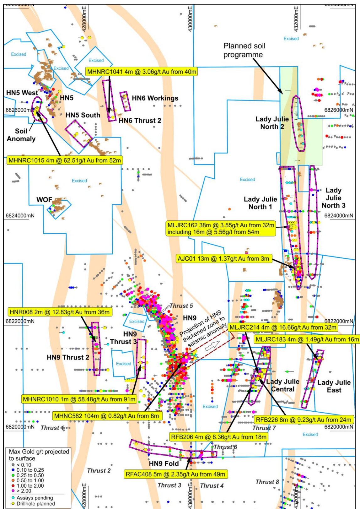
Figure 1 Gold intersection overview covering the HN5, HN6, HN9 and adjacent Lady Julie Projects showing ten additional gold targets covering 14.5km with highlighted intersections (yellow label). Significant historical and Magnetic intercepts (max Au projected to surface) and 40 RC and 4 Diamond holes for 4,264m with assays pending in blue and planned 110 RC holes for 10,310m in yellow.
