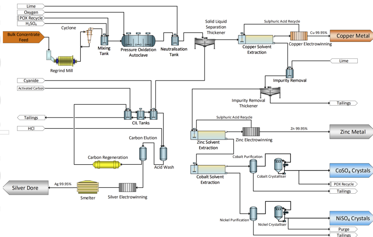
Figure 14: Walford Creek Project process flowsheet – Leaching and metal recovery
