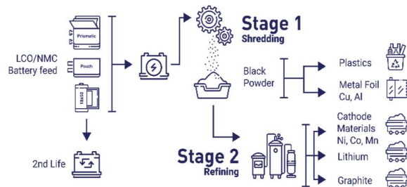
Figure 5 – Process flow diagram showing Front-end Shredding and Beneficiation circuit in the top right
