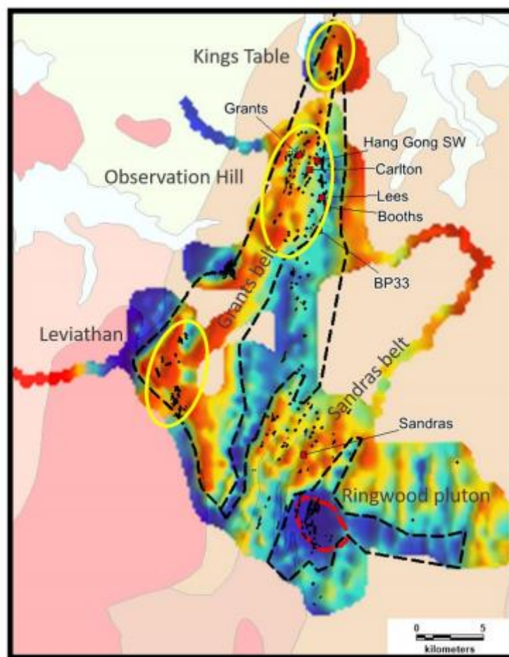
Figure 2 - Residual Gravity Image, Finnis Lithium Project.
