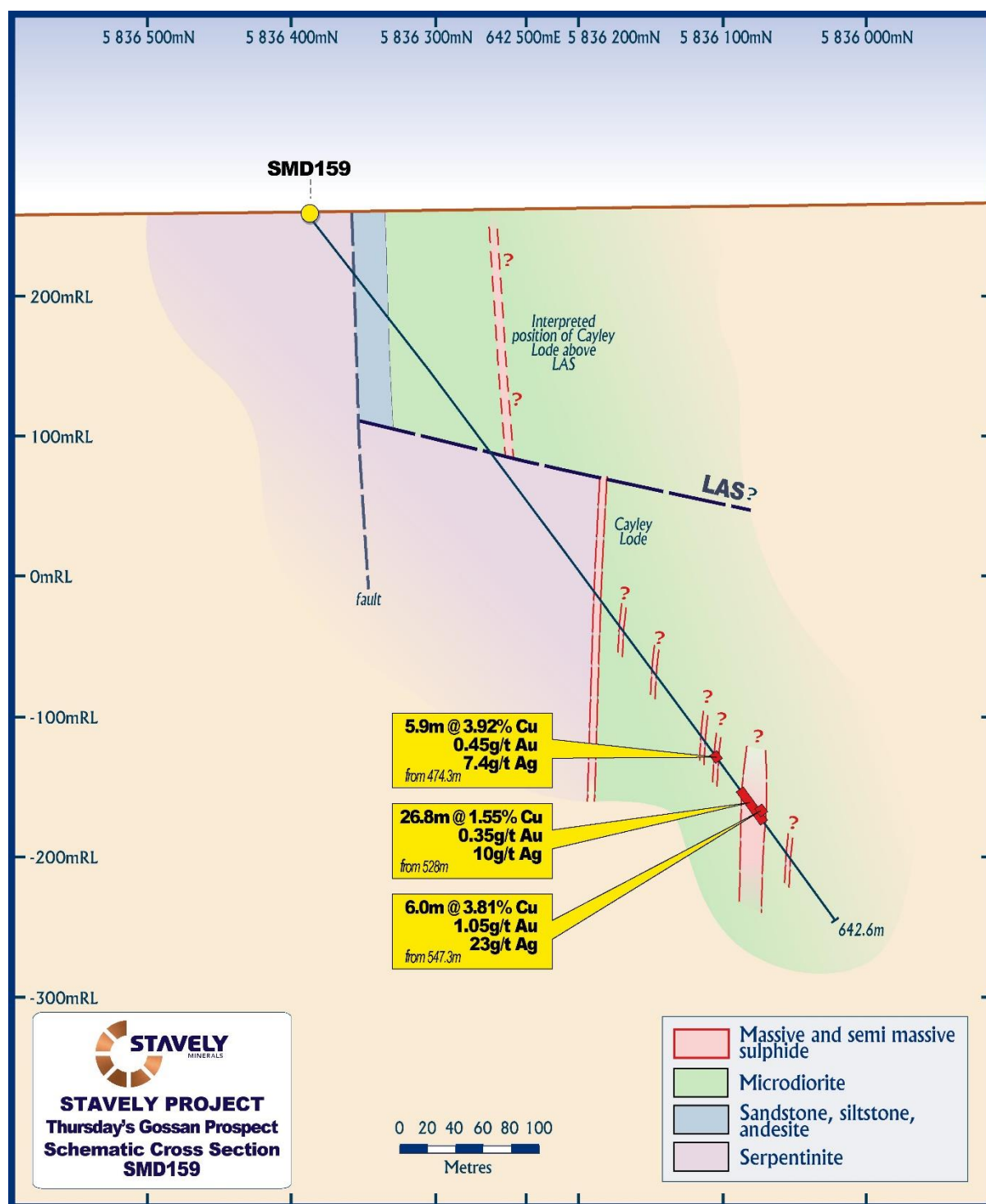
Figure 4. SMD159 drill section.
