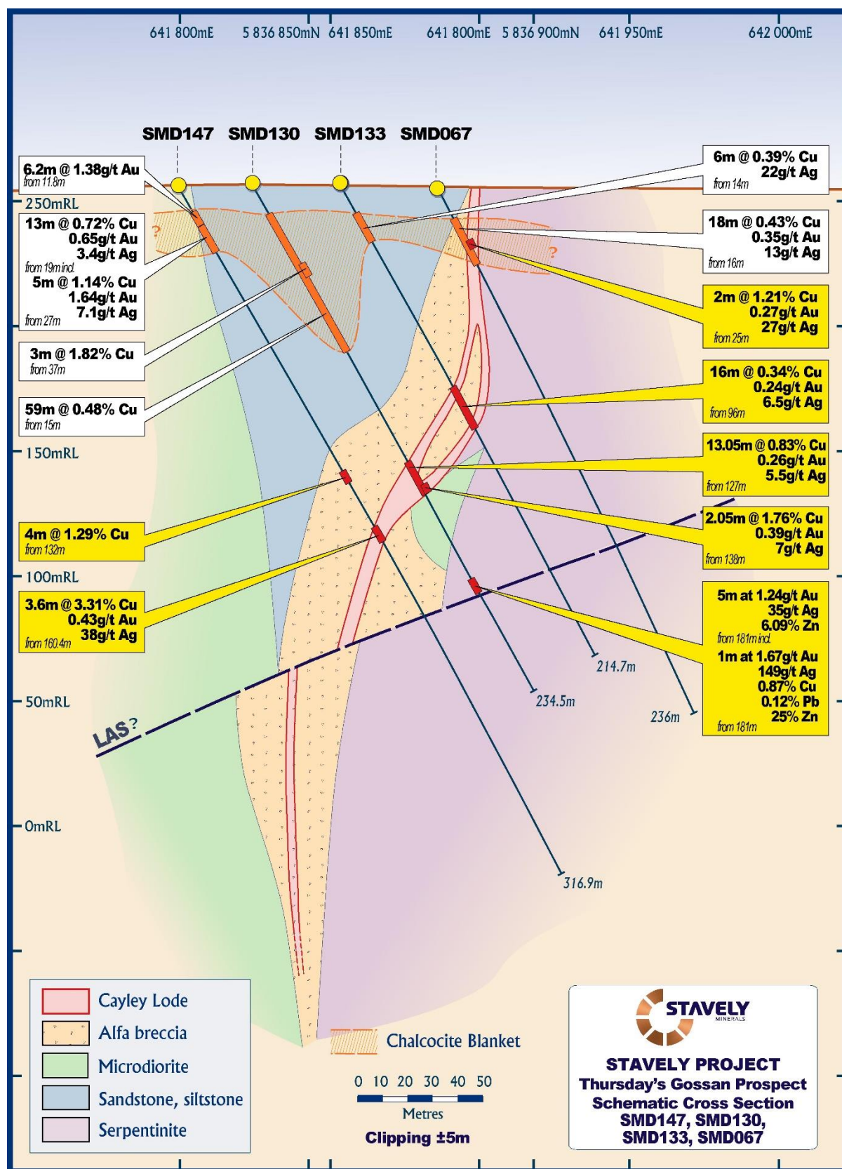
Figure 5. SMD147 drill section.
