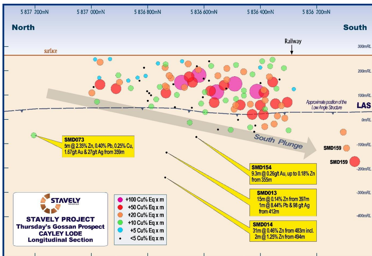
Figure 6. Cayley Lode long section.
