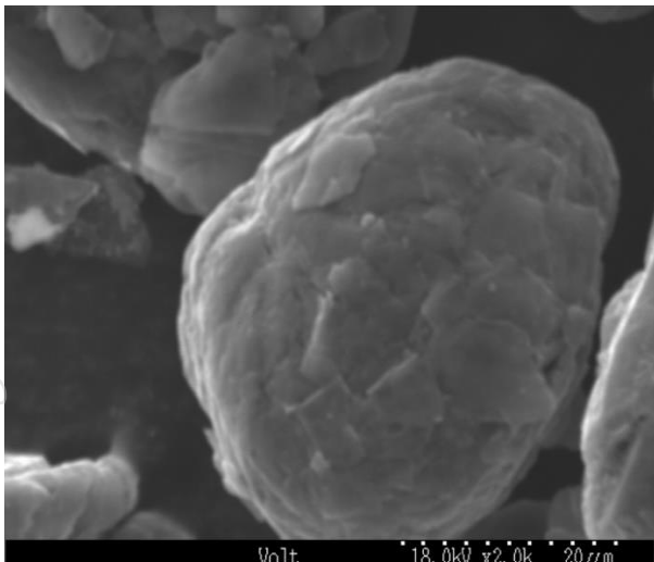
Scanning Electron Microscope (SEM) images of Carbon Coated Spherical Purified (CSPG) Bunyu natural flake graphite
