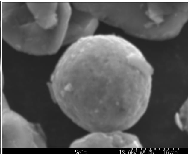
Scanning Electron Microscope (SEM) images of Carbon Coated Spherical Purified (CSPG) Bunyu natural flake graphite
