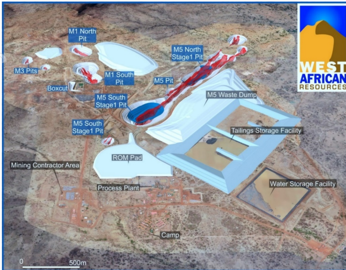
figure 1 - Sanbrado layout
