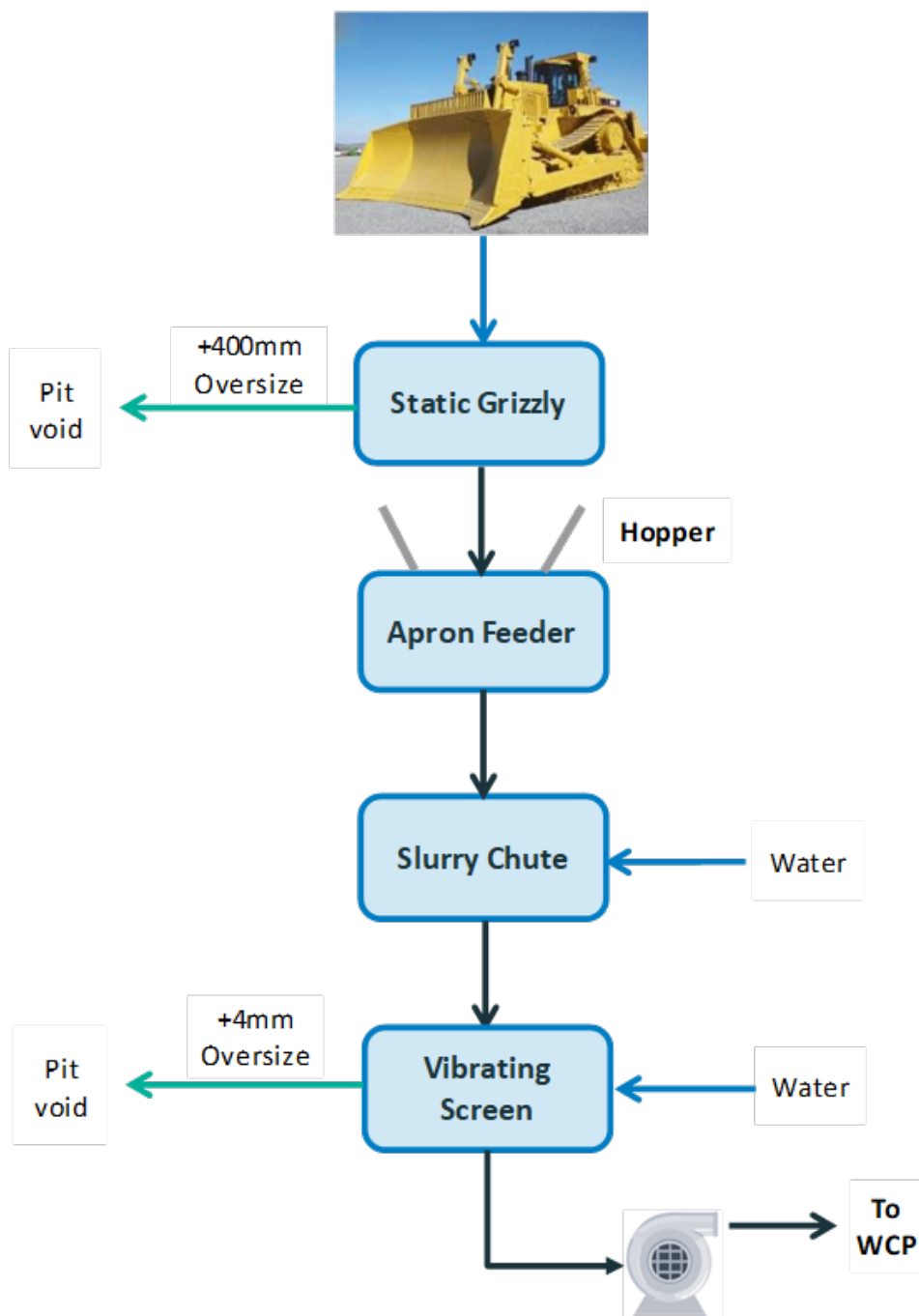
Figure 9: DMU process flow design
