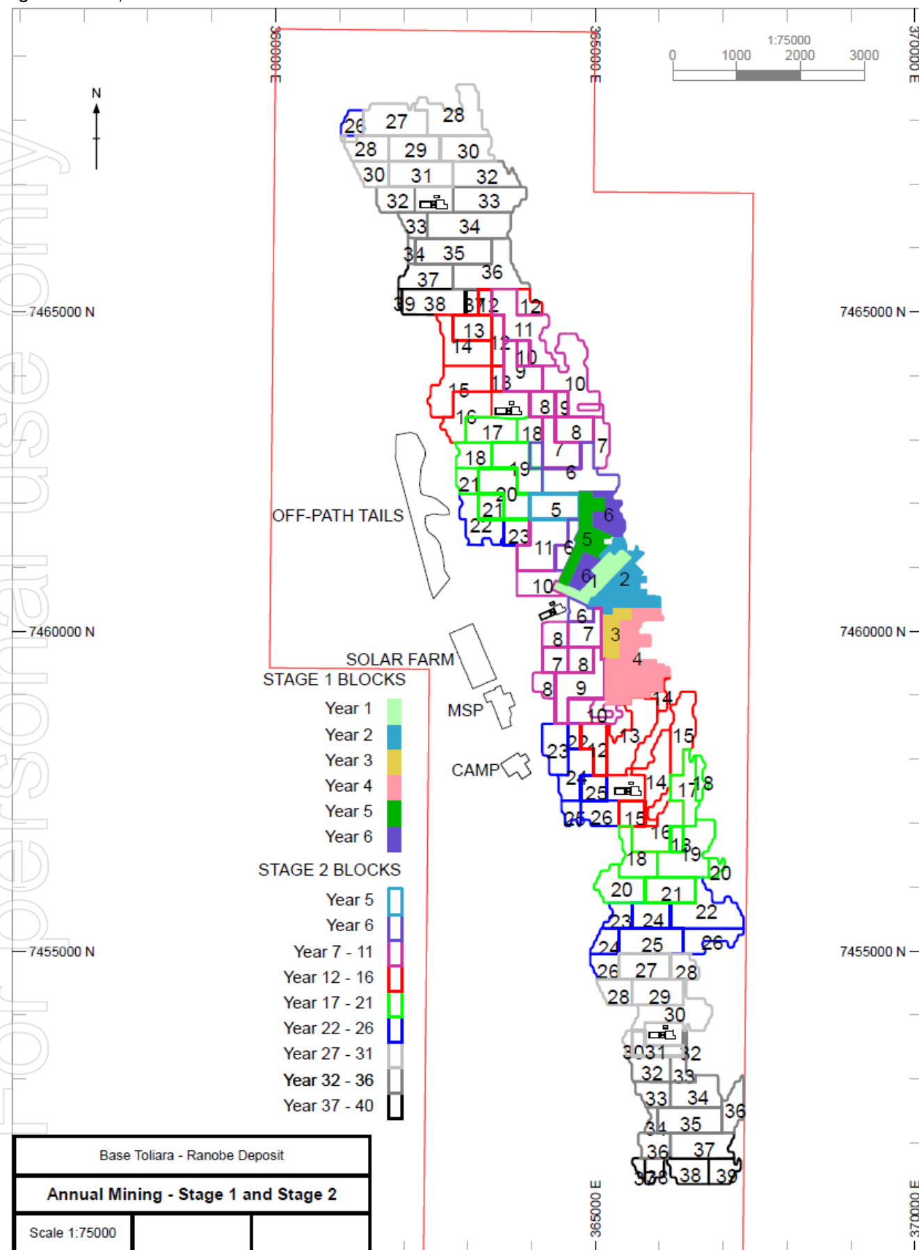
Figure 6: Mine path schedule
