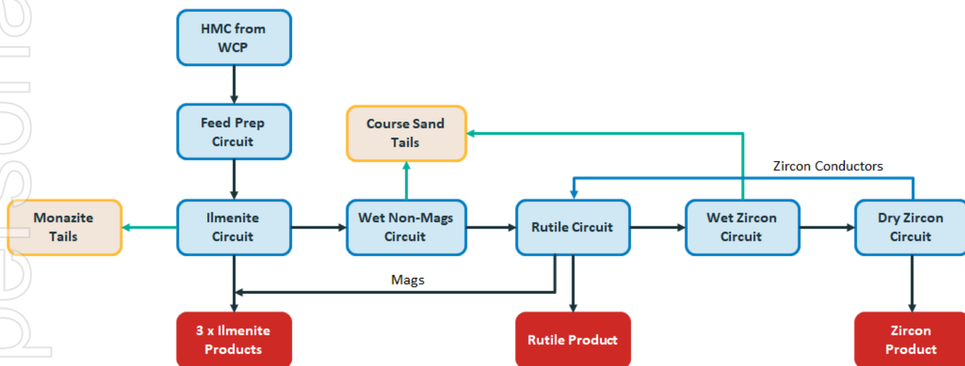
Figure 11: DFS2 MSP process flow design
