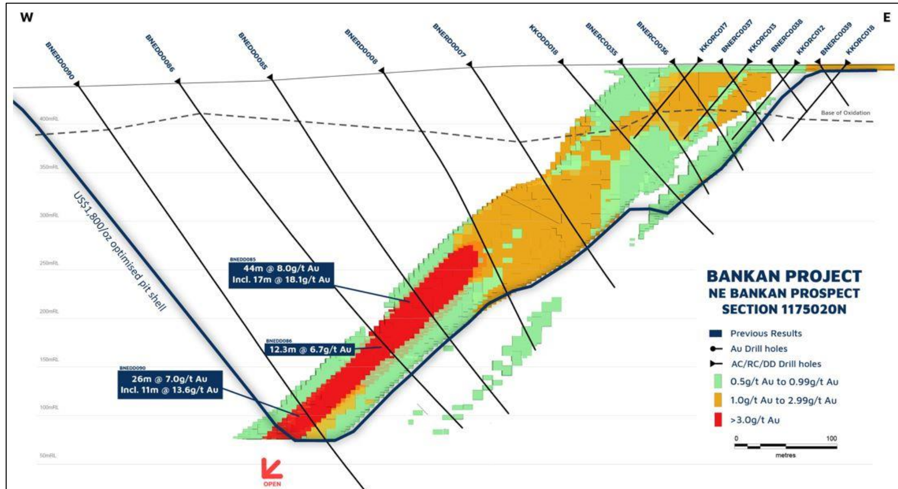
Figure 5 - Cross section 1175,020N illustrating the locations of >3g/t Au blocks (red), plus 1-3g/t Au blocks (dark yellow) and 0.5-1.0g/t Au blocks (green) in the resource model largely within the US$1800/oz gold price-optimised pit shell.
