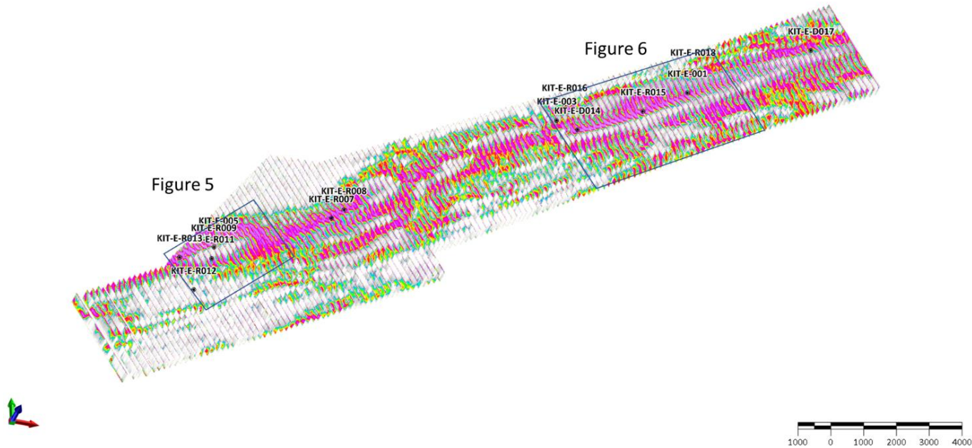
Figure 4. 3D view illustrating completed drilling on AEM layered earth conductivity sections. No vertical exaggeration. Zoom inset areas illustrated in subsequent figures highlighted for context.
