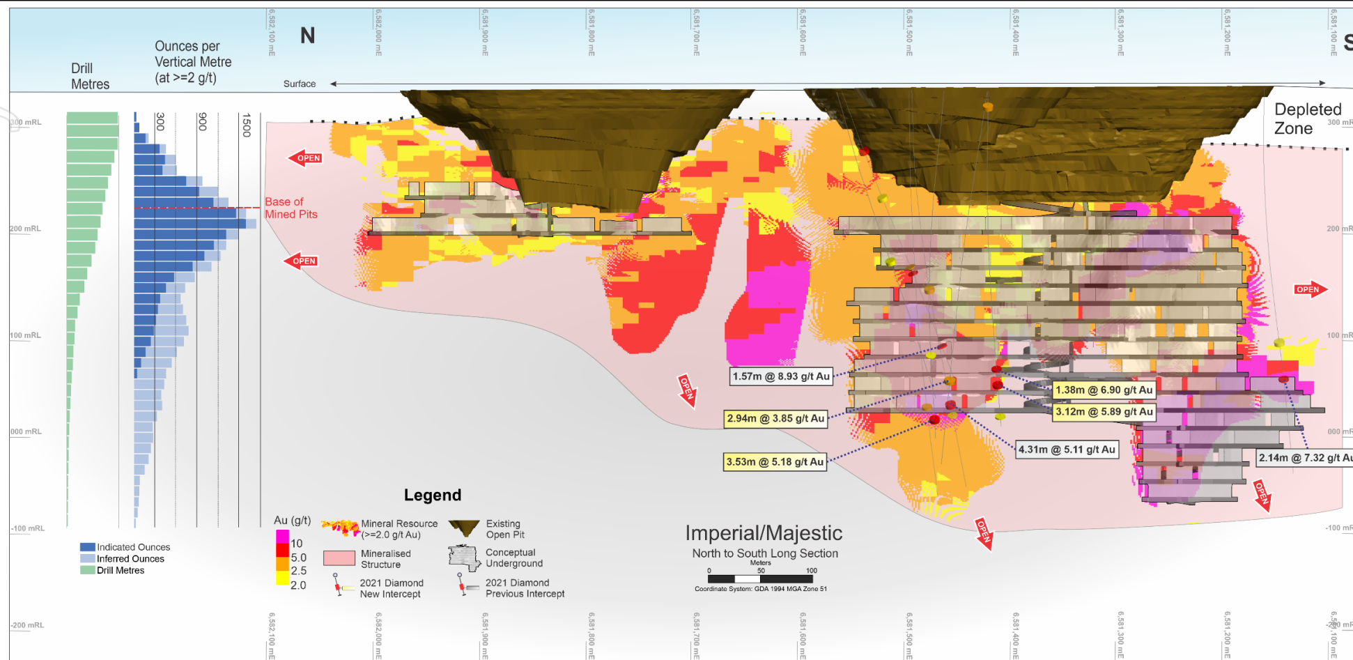
Figure 4: Long section showing Majestic and Imperial. Existing open pits (brown) and Resources > 2.0 g/t Au are shown. Pink shadow indicates < 2.0 g/t Au mineralised structure which remains of interest in a high-grade nuggety system. Planned initial underground development is overlain
