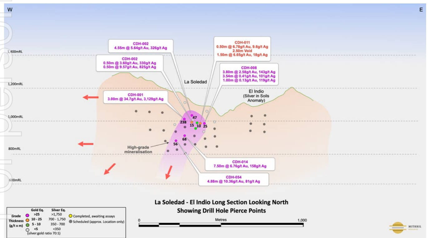
Figure 26: Schematic Long section La Soledad-El Indio with drill hole pierce point for holes completed to date plus conceptual planned resource development holes in turquoise and exploration holes shown in grey. CDH-011 shown in red as a reminder that the void (historic mine workings) Metal equivalent grades calculated using 70 g/t Ag = 1 g/t Au, based on gold price of USD1,610 per ounce and silver price of USD23 per ounce.
