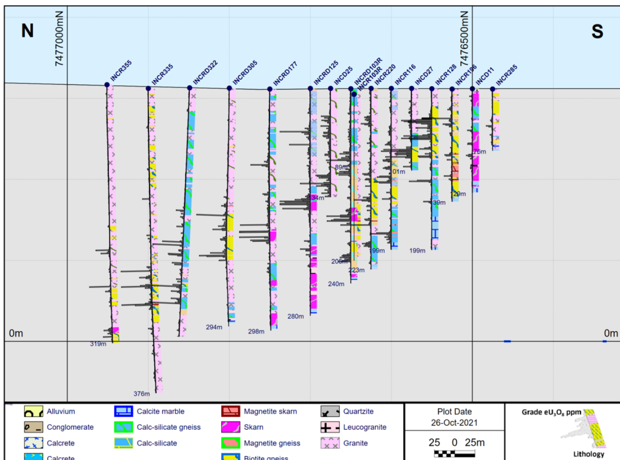
Figure 8: Inca, drill cross-section: 488,950mE/7,477,070mN -- 488,950mE/7,476,330mN
