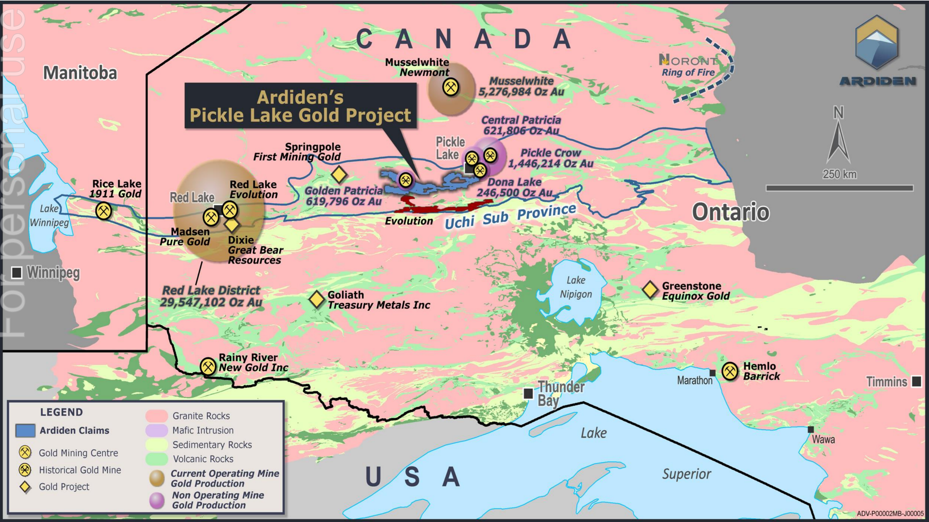
Geological Underlay of the Red Lake to Pickle Lake Archaean Greenstone Belt
