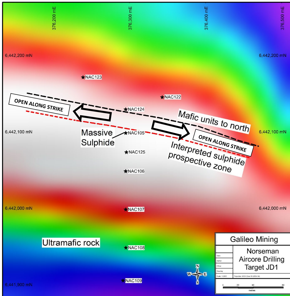
Figure 5 —Aircore drilling on northern edge of JD1 target showing interpreted sulphide zone on contact between ultramafic and mafic rock units (over TMI magnetic image)
