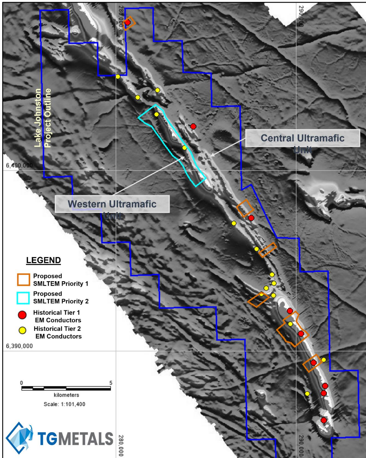
Figure 1 – Aeromagnetic Image with location of priority targets for ground geophysics and drilling Datum: AMG Zone 51 (AGD84)
