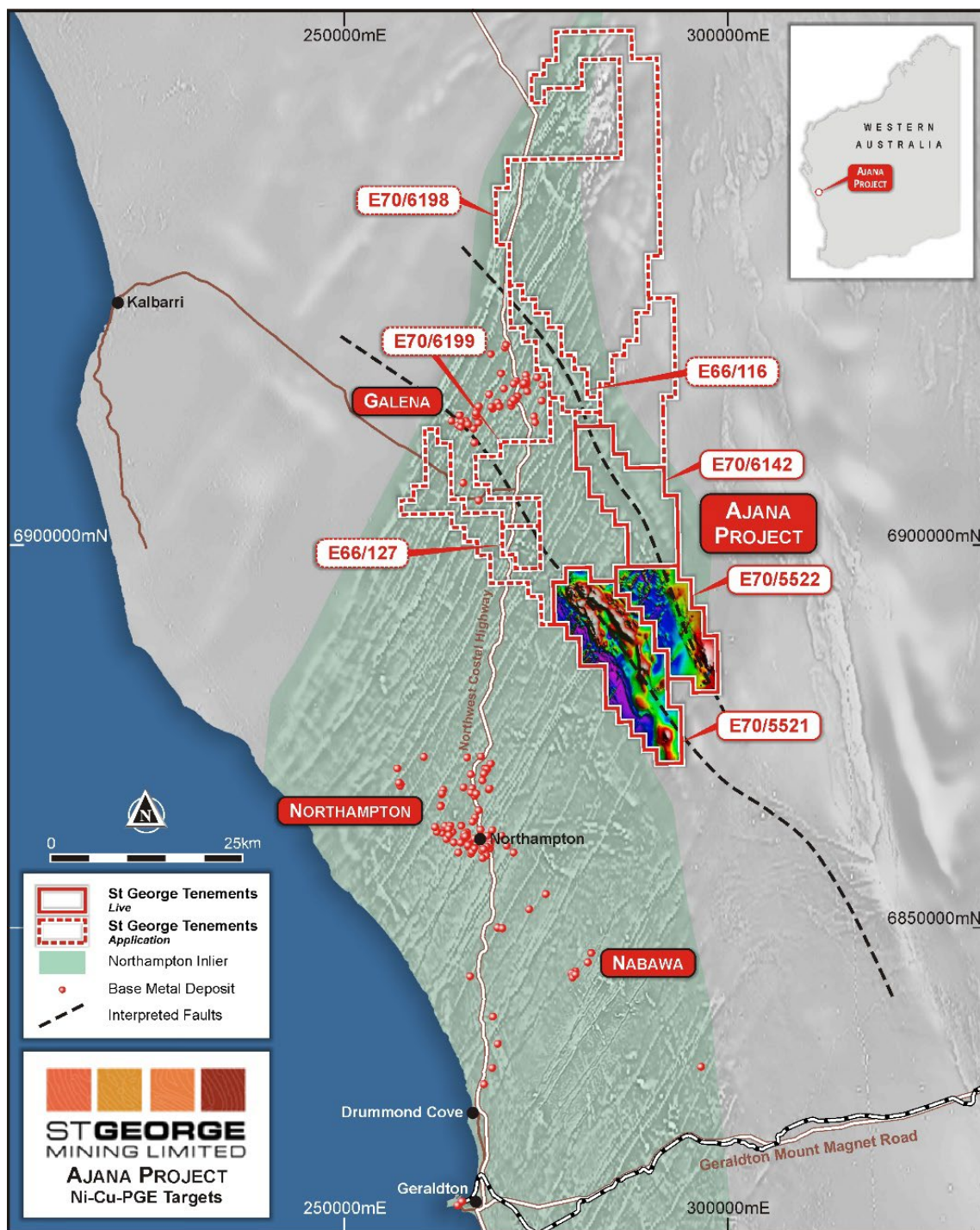
Figure 6: St George's Ajana Project (against magnetic RTP 1VD) showing the Northampton Mineral Field highlighted green and the location of historic base metal deposits and mines.
