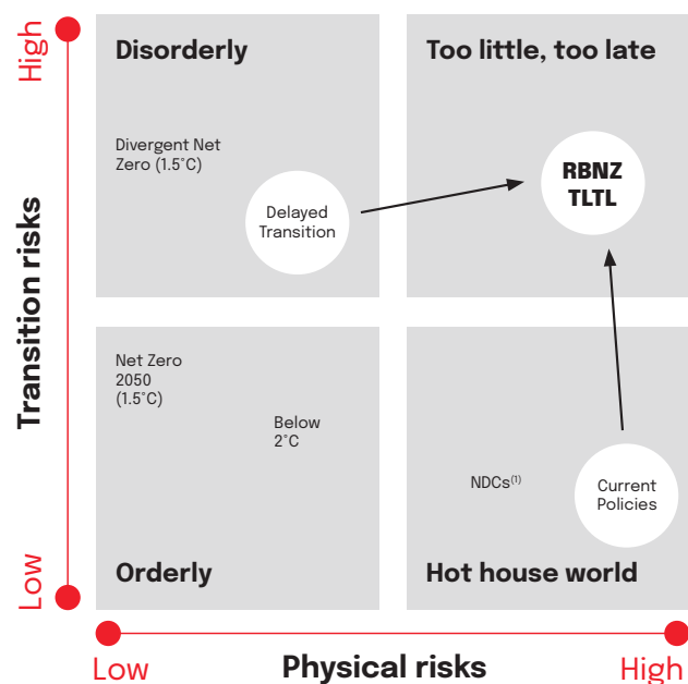
Figure 6: NGFS scenario framework
