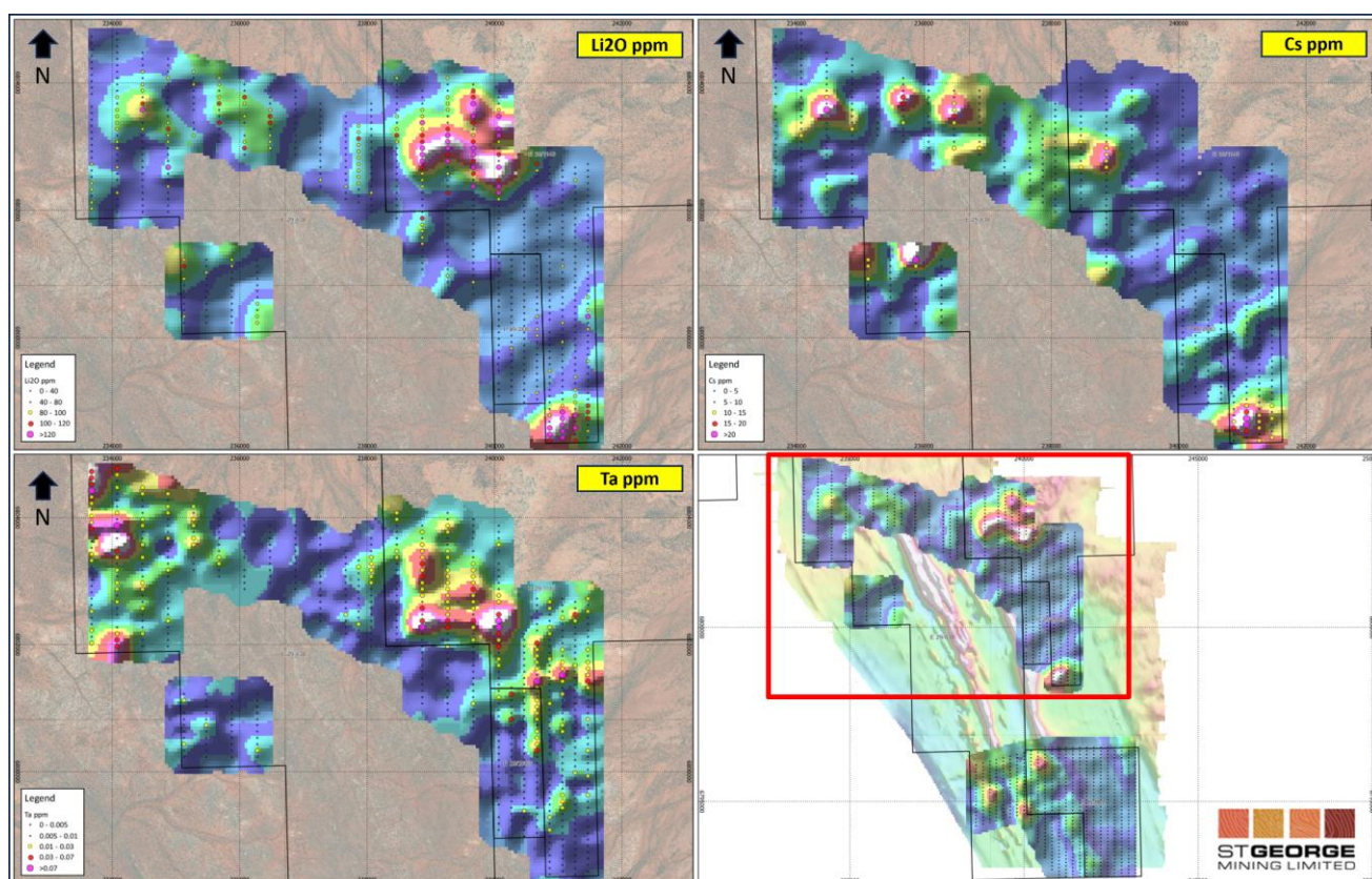
Figure 5 – plots showing the strong coincidence of the lithium, caesium and tantalum soil geochemistry in the northern survey area.
