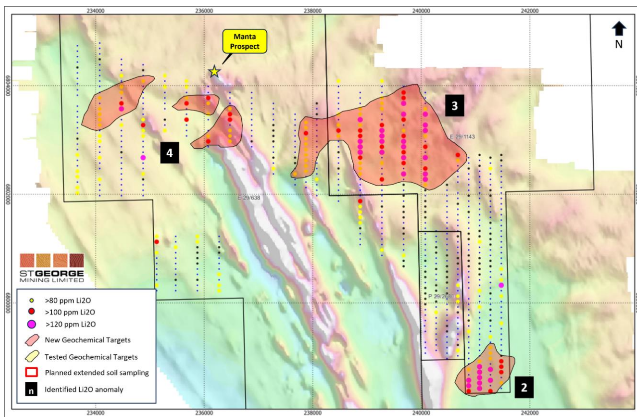
Figure 4 – soil anomalies in the northern survey area.
