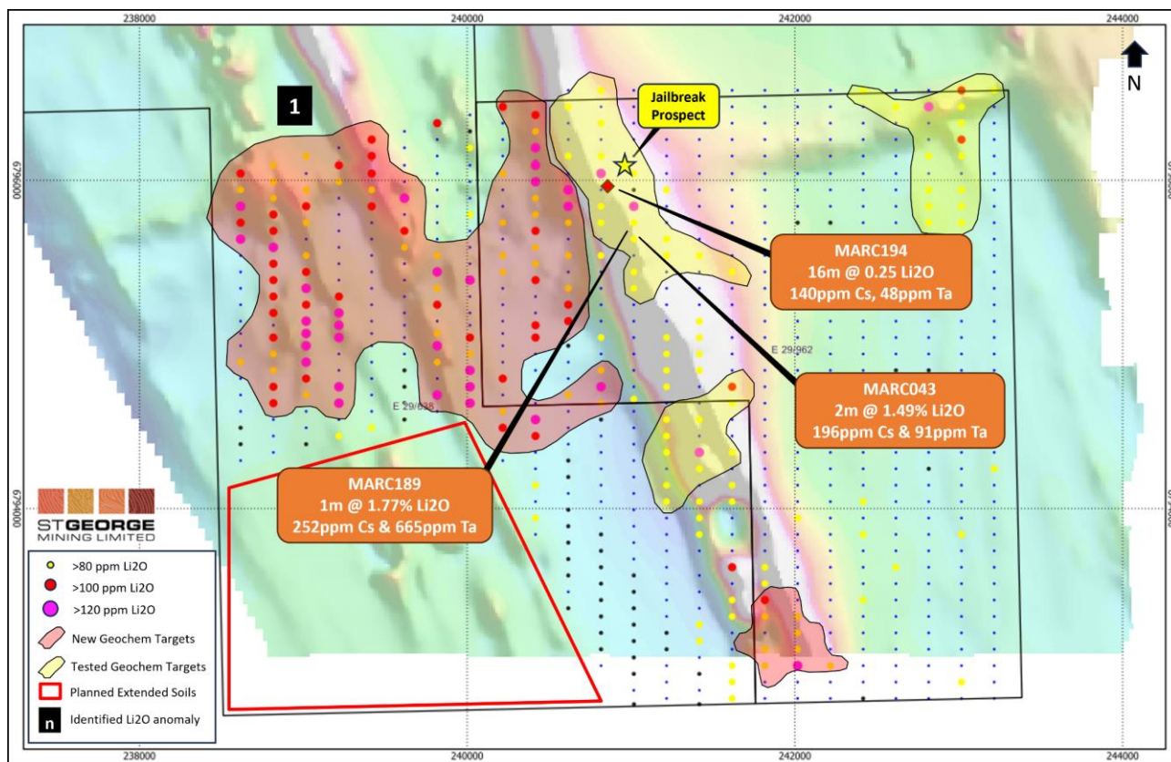
Figure 6 – soil anomalies in the Jailbreak West survey area.
