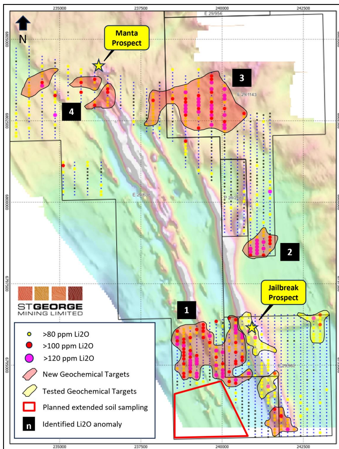
Figure 2 – map of Mt Alexander (overlying magnetic data) showing lithium in soil anomalies.
