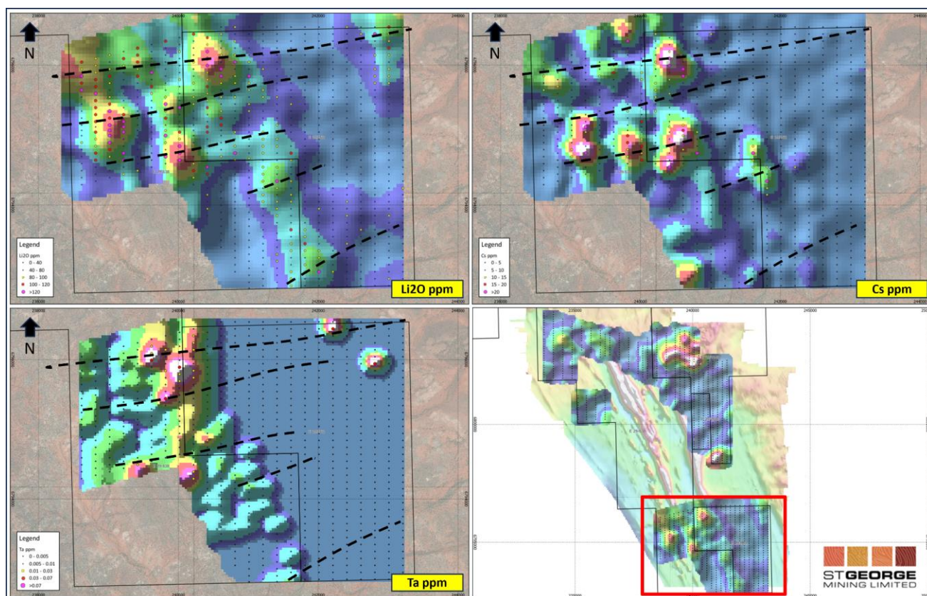
Figure 7 – plots showing the strong coincidence of the lithium, caesium and tantalum geochemistry in the Jailbreak west survey area.
