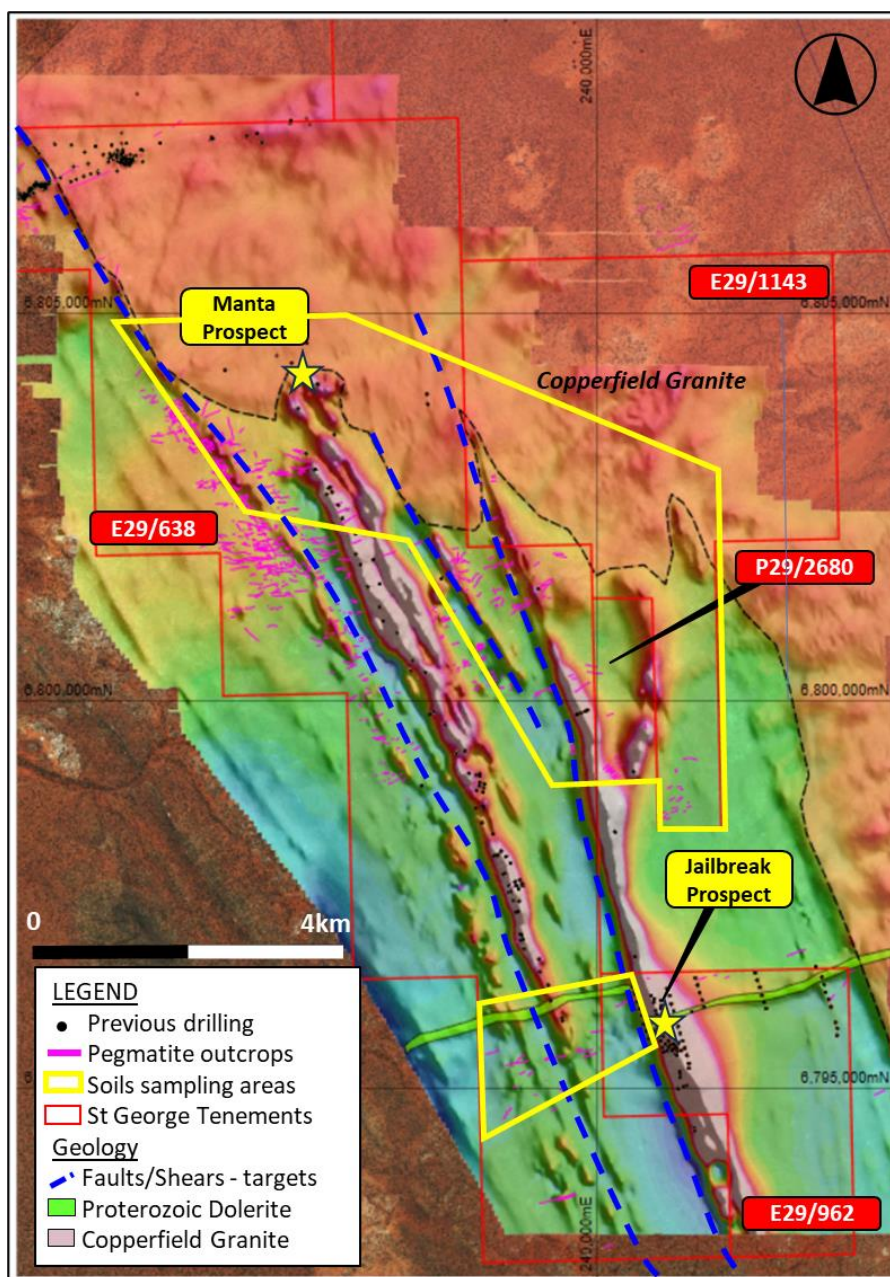
Figure 1 – Mt Alexander Project map showing soil survey areas and the interpreted contact between the greenstone sequence and the Copperfield Granite overlying TMI magnetics imagery.
