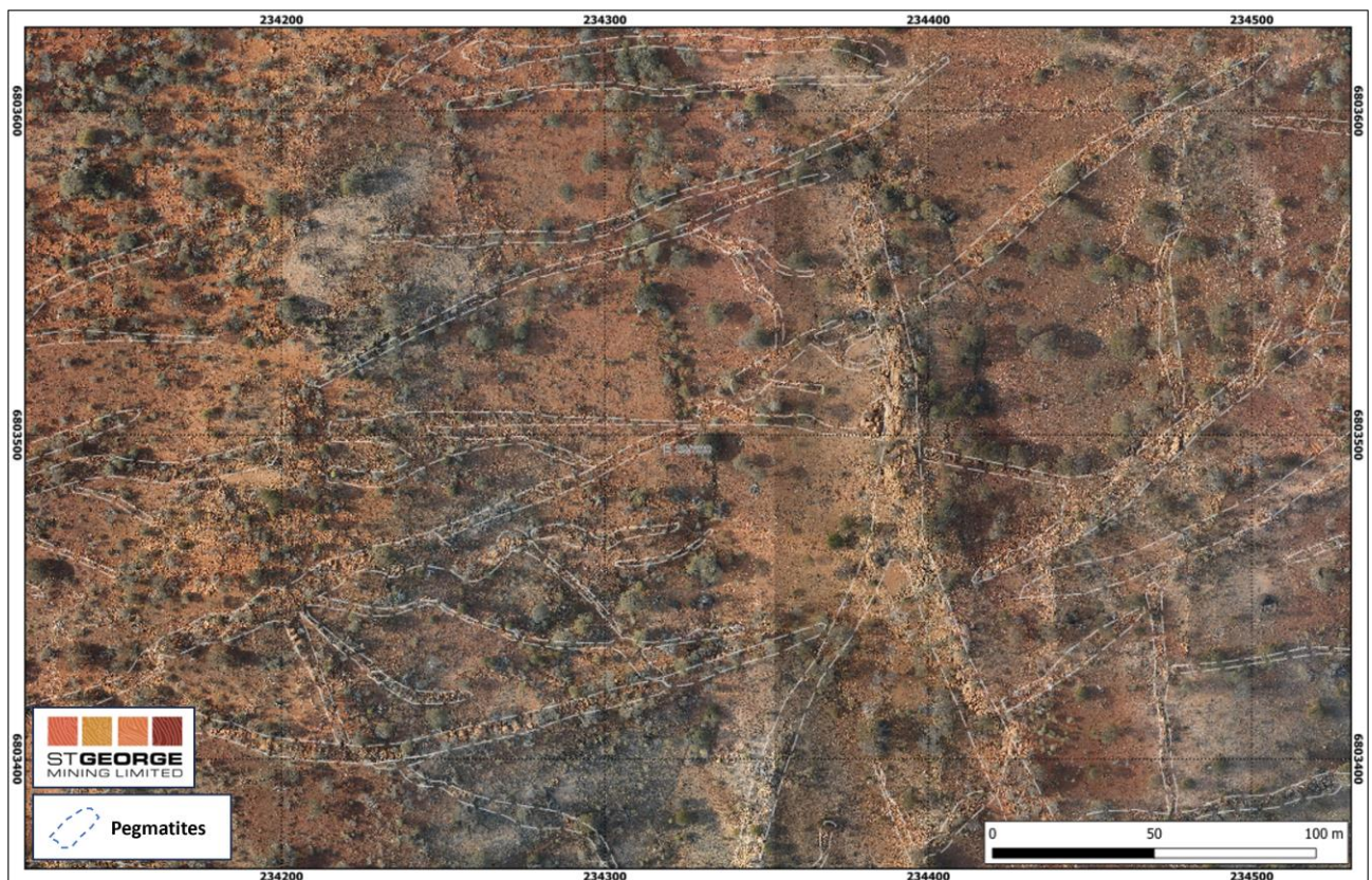
Figure 3 – drone imagery showing an example of pegmatite outcrop at Target 4.
