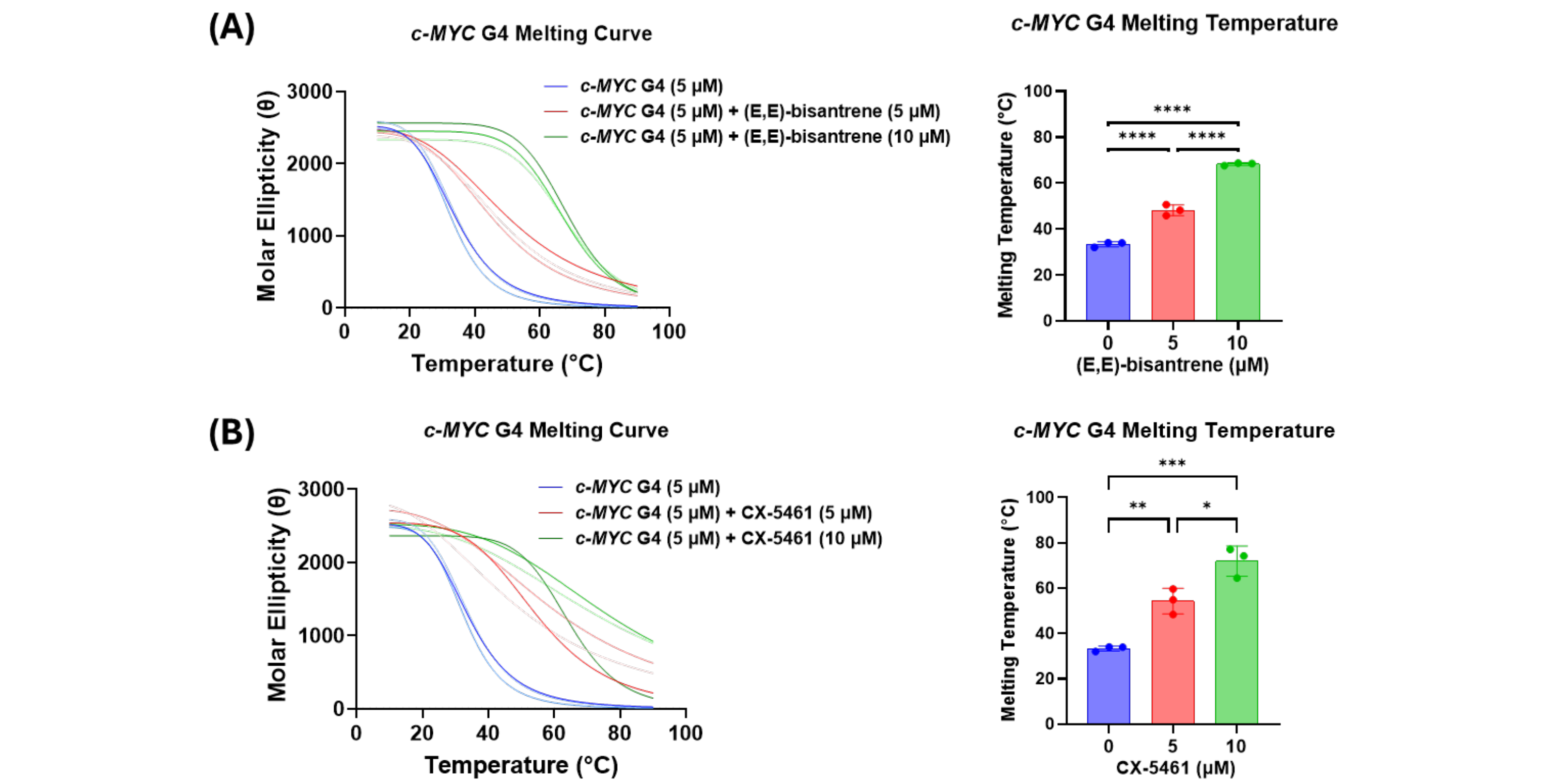
Figure 4: Melting curves of c-MYC G4 DNA sequence in the presence of (E,E)-bisantrene (A) or CX-5461 (B). Molar ellipticity for c-MYC G4 was determined at 265 nm using circular dichroism spectroscopy.
