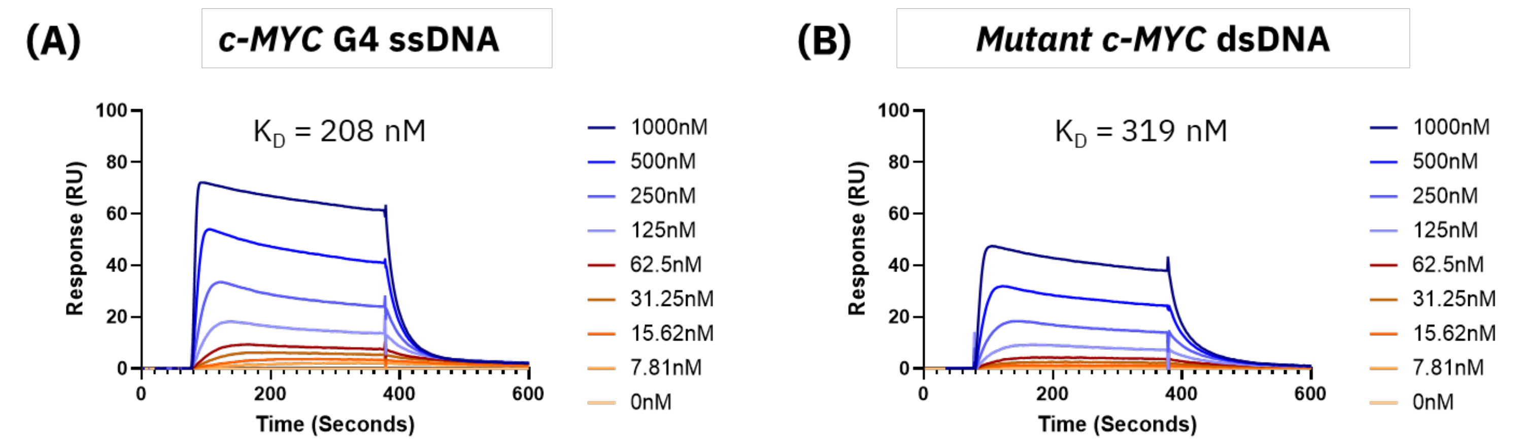
Figure 3: SPR analysis of (E,E)-bisantrene binding to 1000 response units (RU) of: (A) c-MYC G4 ssDNA (5'-/5Biosg/TGAGGGTGGGTAGGGTGGGTAA-3'), and (B) a related mutant c-MYC dsDNA sequence (5'-/5Biosg/TGAGAGTGAGTAGAGTGAGTAA-3' and 5'-TTACTCACTCACTCACTCA-3') on a NeutrAvidin-coated sensor chip. (E,E)-bisantrene was injected in a concentration series from 0–1000 nM over multiple sequential injections, each lasting 300 s at a flow rate of 25 μL/min, followed by a 600 s dissociation phase.
