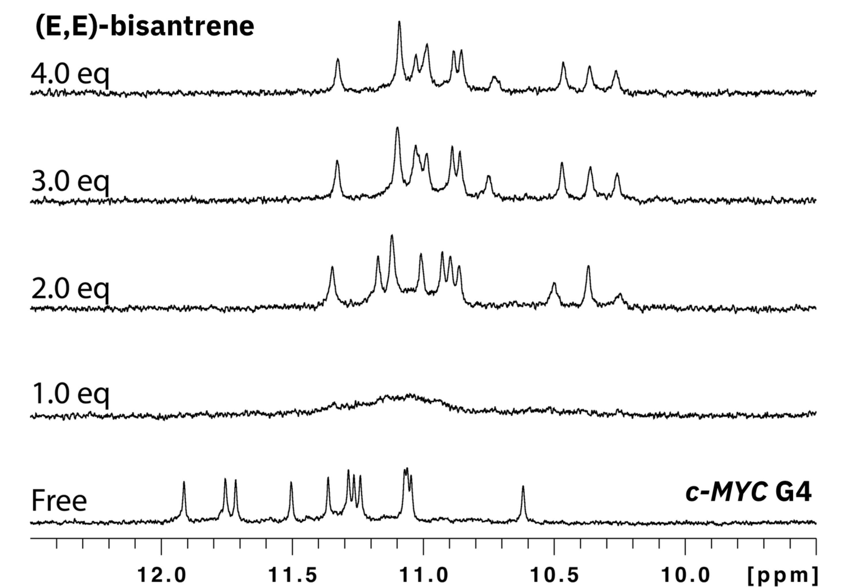
Figure 1: 1 H-NMR titration (guanine imino proton region) of c-MYC G4 DNA with (E,E)-bisantrene. Conditions: 100 mM K + , pH 7.0, 25°C; DNA concentration, 150 μM; ratios of (E,E)-bisantrene/c-MYC G4 are shown.
