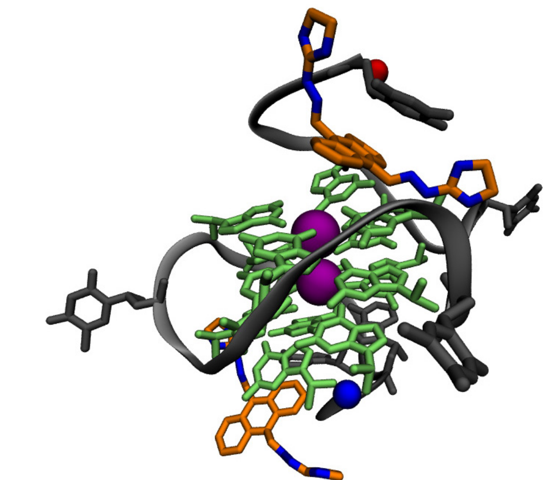
Figure 2: Representative binding mode (34.9% population) of (E,E)-bisantrene (orange sticks) interaction with the c-MYC G4 (PDB ID: 2MGN). 5' and 3' ends of the DNA chain are indicated by red and blue spheres, respectively. K + ions are indicated by purple spheres.
