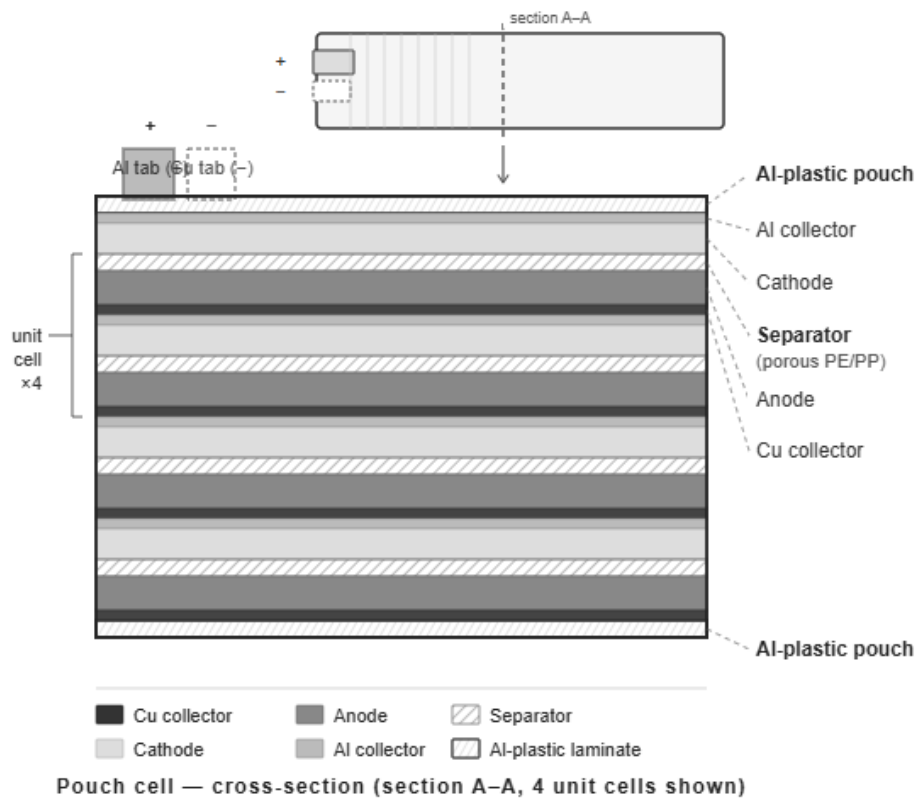
Figure 1: Schematic LiB cross-section of a pouch cell format LiB showing anode, cathode and separator.
