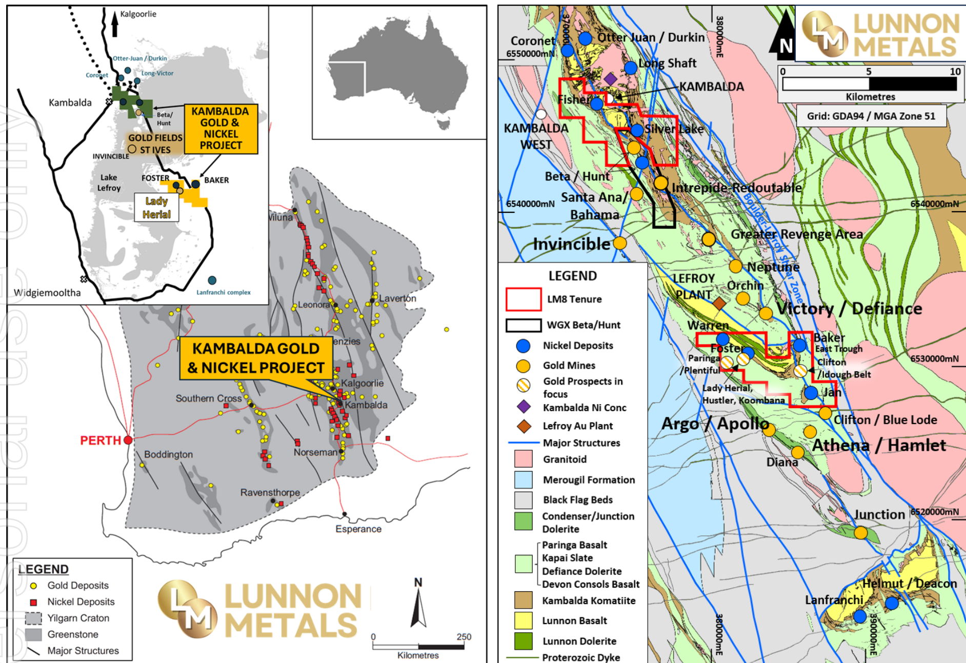
Figure 2: Location of the KGNP, regionally and at the local Kambalda/St Ives scale; showing surface geology and structure of this significant Australian gold camp.
