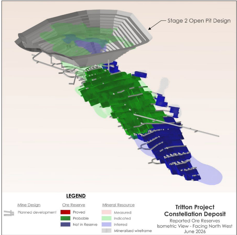
Figure 25: Constellation Underground Maiden ORE mine design
