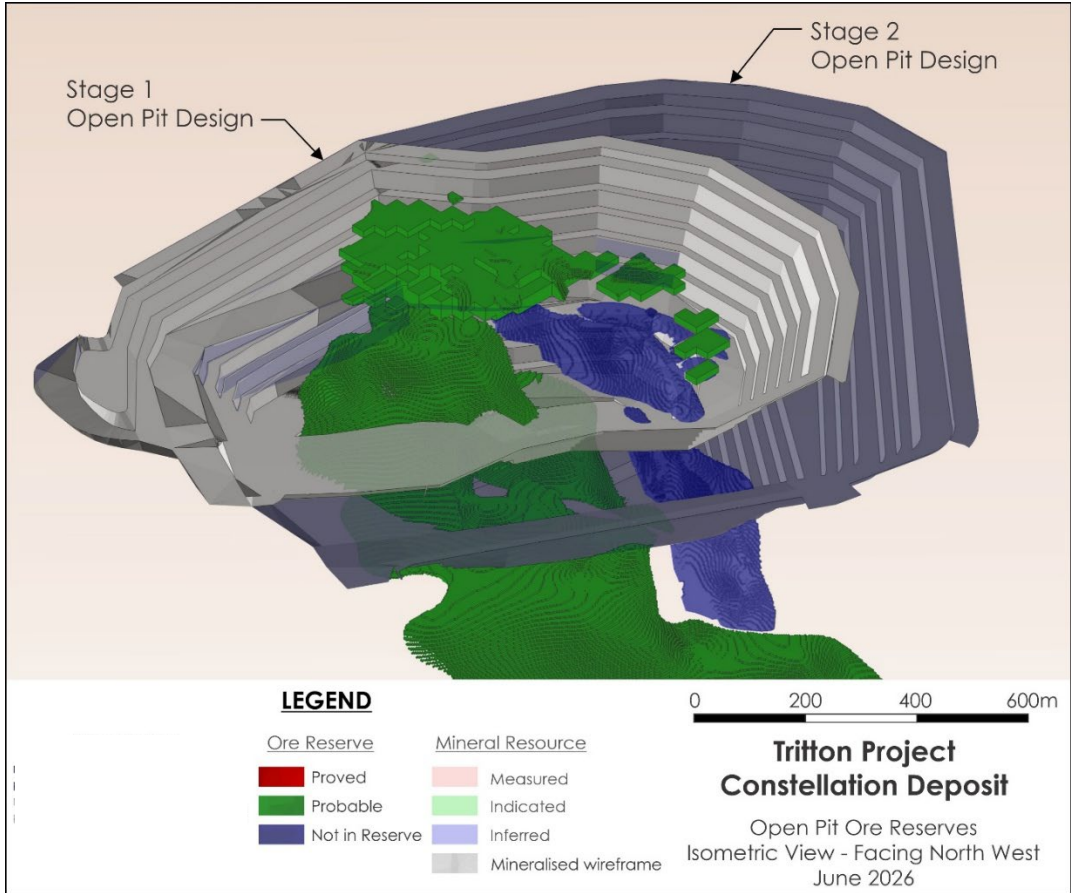
Figure 24: Constellation Open Pit ore reserve mine design
