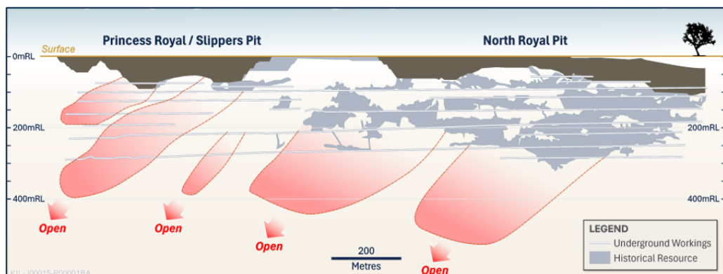
Figure 3: Plan and long-section comparison of New Waverley and Pantoro Limited's Royal Group deposits, highlighting the scale and vertical extent of the Royal Group reef system relative to the limited shallow drilling at New Waverley, which remains open along strike and at depth. Royal Group information sourced from Pantoro Gold Diggers and Dealers 2020 & 2025 presentations, and ASX announcement dated 25 November 2025.
