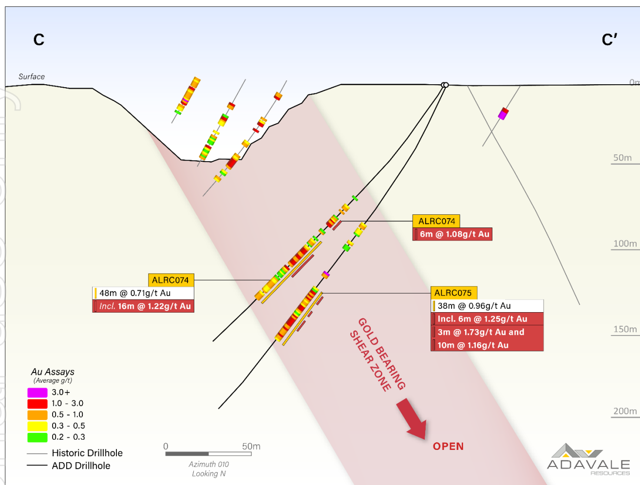
Figure 2: Cross Section Displaying position and gold results for ALRC074 and ALRC075 relative to the historic London-Victoria Open Pit (Section Line C-C' displayed in Figure 1) ALRC074 interval 48m @ 0.71g/t Au is calculated with 0.3g/t cut-off and 4m internal dilution
