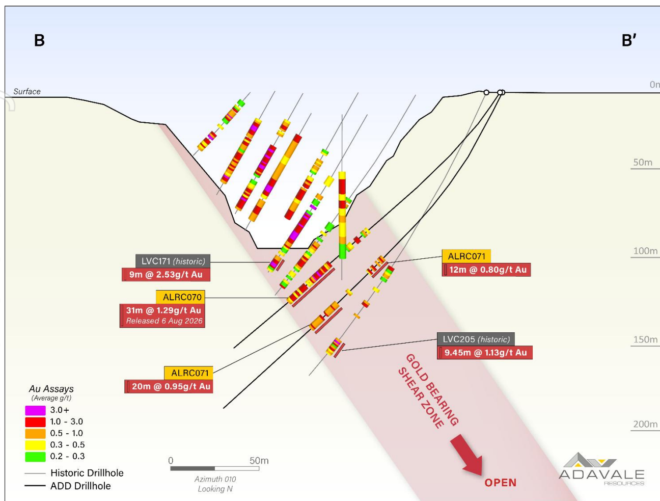
Figure 4: Cross Section Displaying position and gold results for ALRC071 and ALRC070 (released 6 August) relative to the historic London-Victoria Open Pit (Section Line B-B' displayed in Figure 1)
