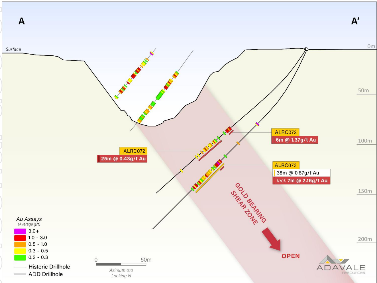
Figure 3: Cross Section Displaying position and gold results for ALRC072 and ALRC073 relative to the historic London-Victoria Open Pit (Section Line A-A' displayed in Figure 1)
