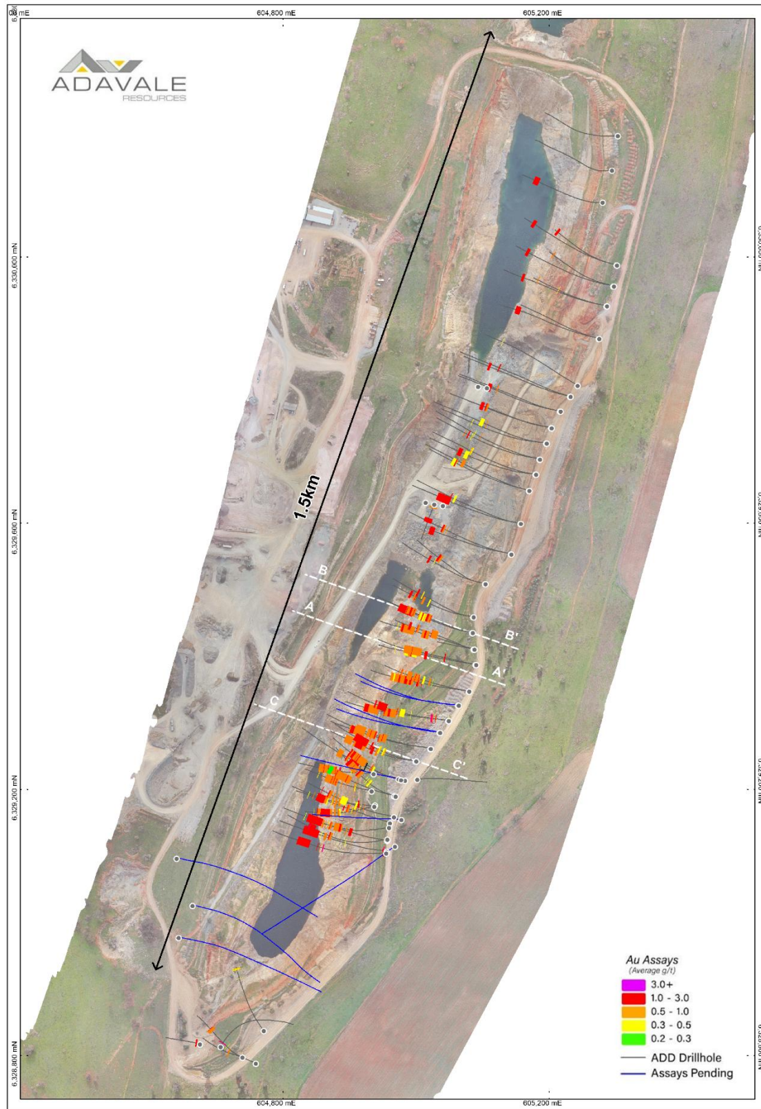
Figure 1: Plan View of the London Victoria Open Pit displaying all Adavale Drillholes to date (projected to surface) coloured with calculated gold intervals >1m wide over 0.3g/t Au projected to surface.
