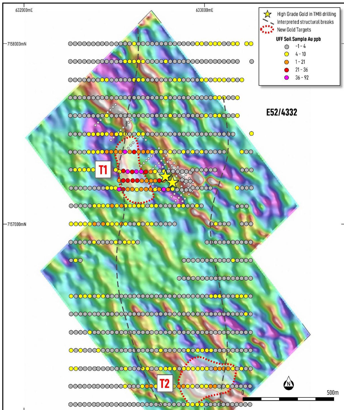
Figure 1: Location plan showing Beatty Park Sth prospect and T2 gold-in-soil anomaly 2 on SAM (sub-audio magnetic) MMT 1VD image (MGA94 zone 50).
