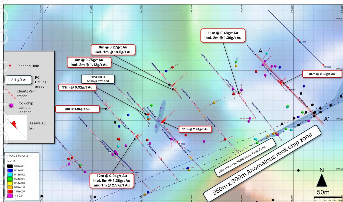
Figure 3 Clifton East plan view showing existing rock chips 2 and recent drill hole traces, previously reported assay intervals 3 and planned drilling, collars shown in red. Background in RTP-TMI magnetic image.
