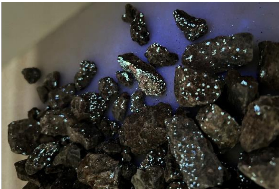
Figure 1; High grade sorted fraction (Set 1) from the Conquest Pit sample LKMET0006 under ultraviolet light, showing characteristic blue-white fluorescence of scheelite. This fraction returned an assay of 1.91% WO 3 , approximately 3.1x the calculated raw feed grade (refer Table 1).
