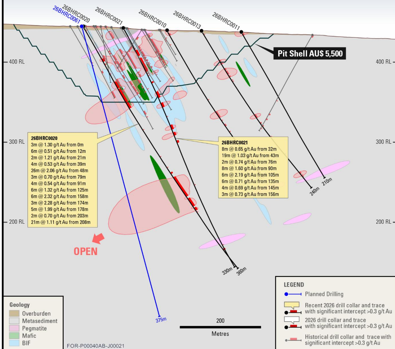
Figure 3. Cross Section B to B 1
