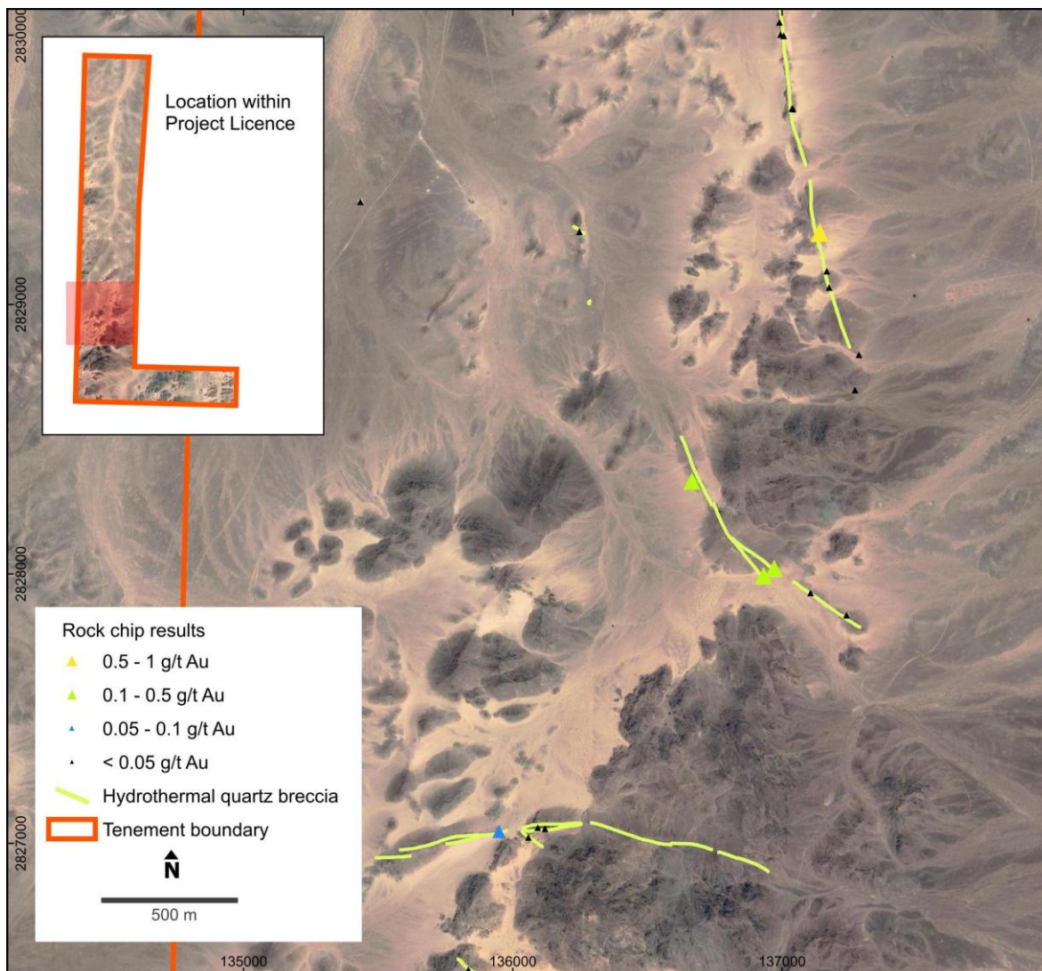
Figure 6 Mapped veins and rock chip sample locations at Wadi Ash Shuwayla license area
