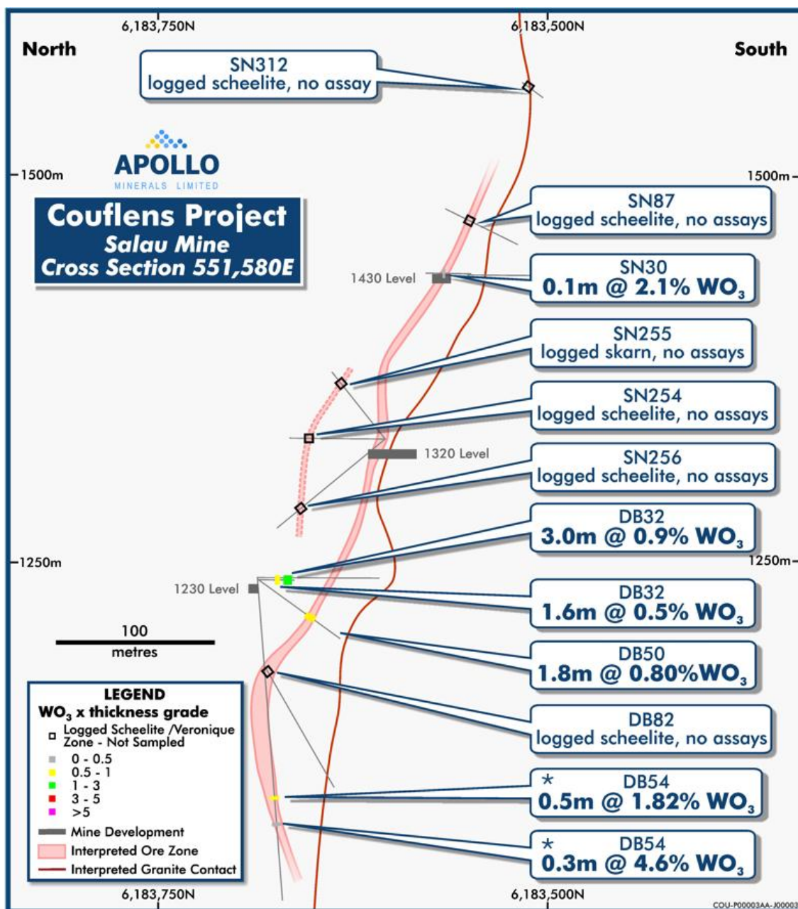
Figure 2: Salau Mine cross section 551,580mE of Veronique Upper Zone: – Displaying interpreted mineralisation trends and historical drillhole data (* previously released intercept – 9 April 2026).
