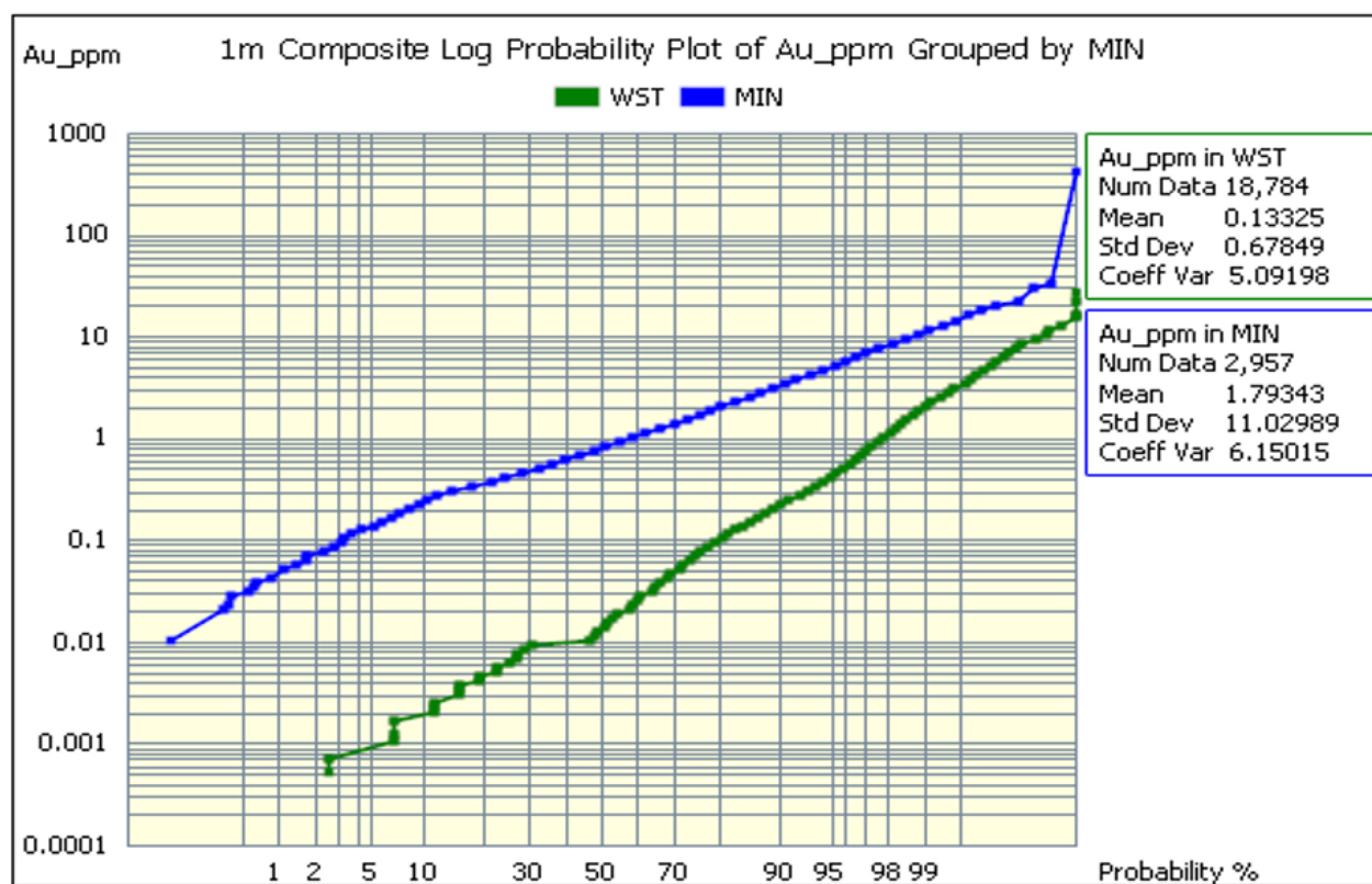
Figure 7: Au Log Probability Plot by Domain
