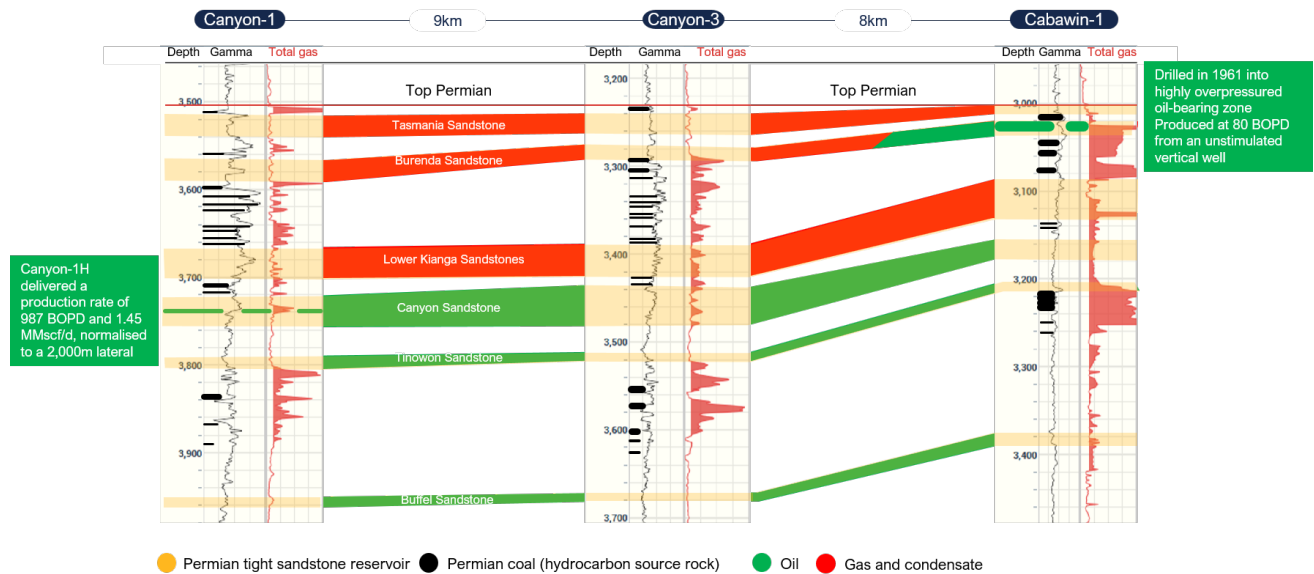
Figure 4: Geological correlation between Canyon-1, Canyon-3 and Cabawin Oil Field
