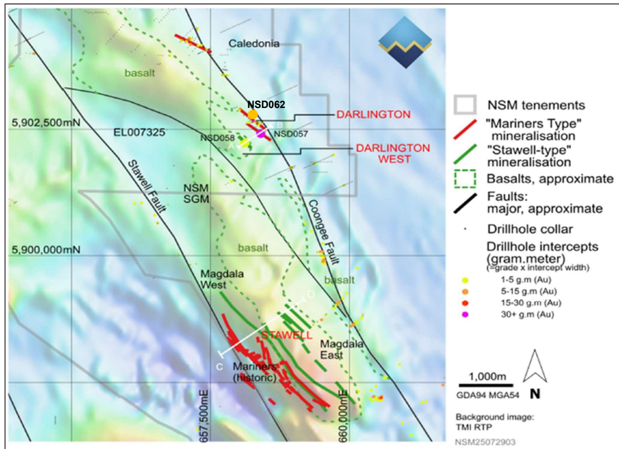
Figure 3 The Darlington-Caledonia trend, north of Stawell, is interpreted as the far-northern continuation of the Magdala Basalt that controls and hosts the deposit at Stawell.
