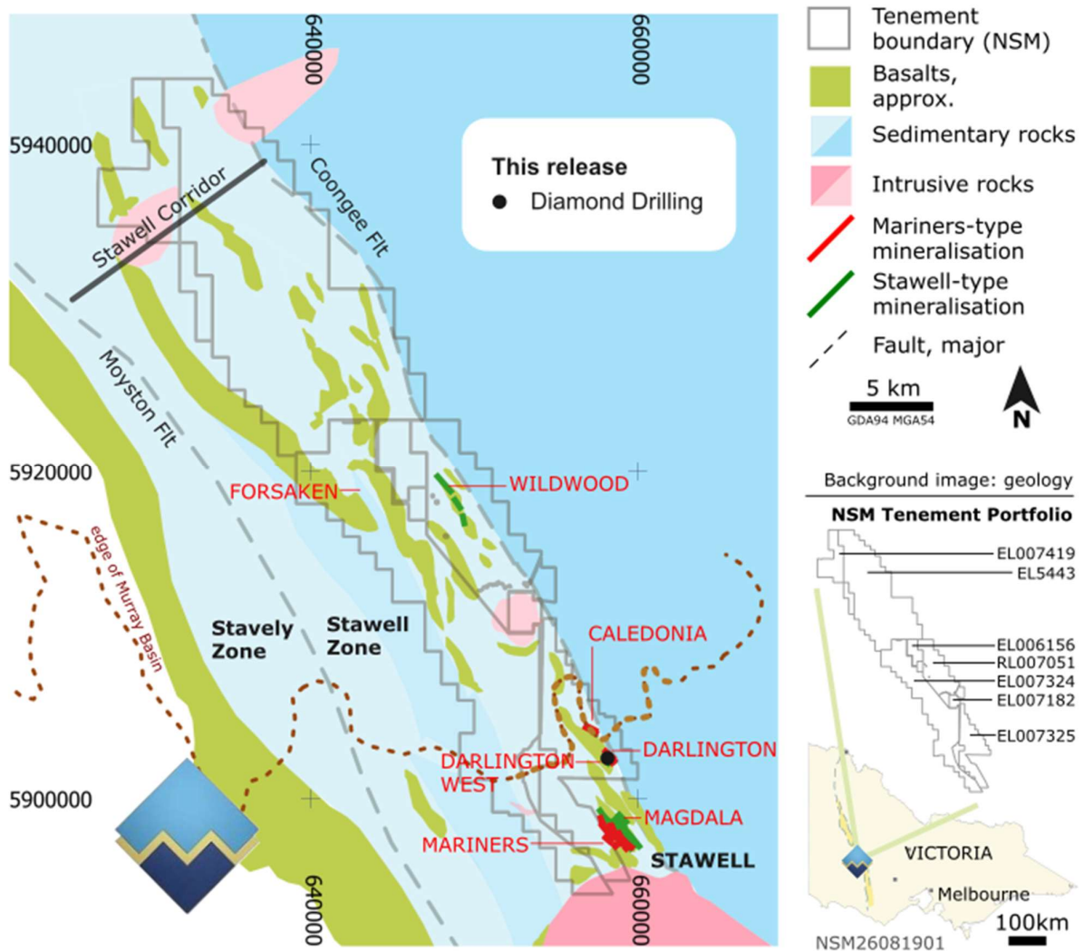
Figure 2 The Stawell Corridor. Gold mineralisation occurs on the margins of, or above, slabs of basalt (shown green). Current NSM exploration activities are focused on the Darlington-Caledonia and Wildwood prospects. However, all basalts within the project area are considered prospective for both Stawell-type and Mariners-type gold mineralisation, based on exploration models developed from the multi-million ounce gold mine at Stawell.
