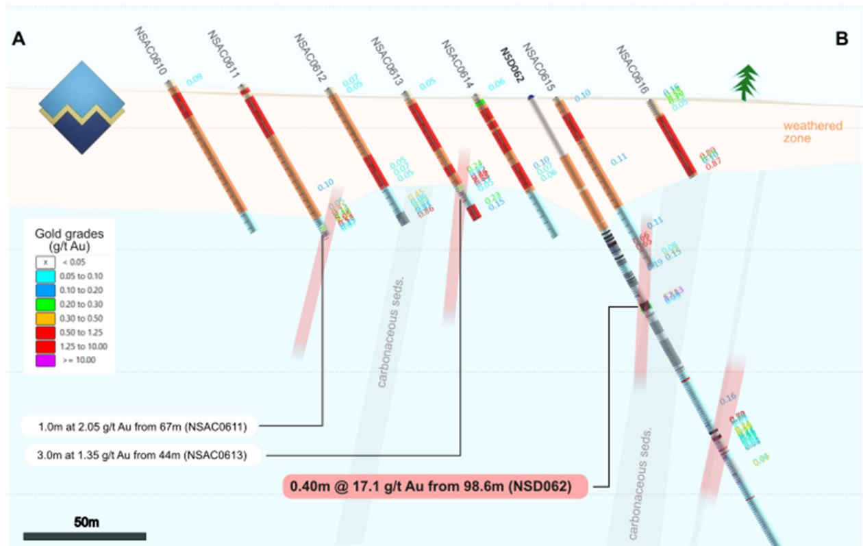
Figure 5 Cross section, NSD062 with interpreted geology and mineralisation. NSD062 targets beneath anomalous gold values in recent air core drilling along strike from previous high-grade gold intercepts. (ASX:NSM 2 July 26). Additional air core results are interpreted as an additional zone, untested at depth.
