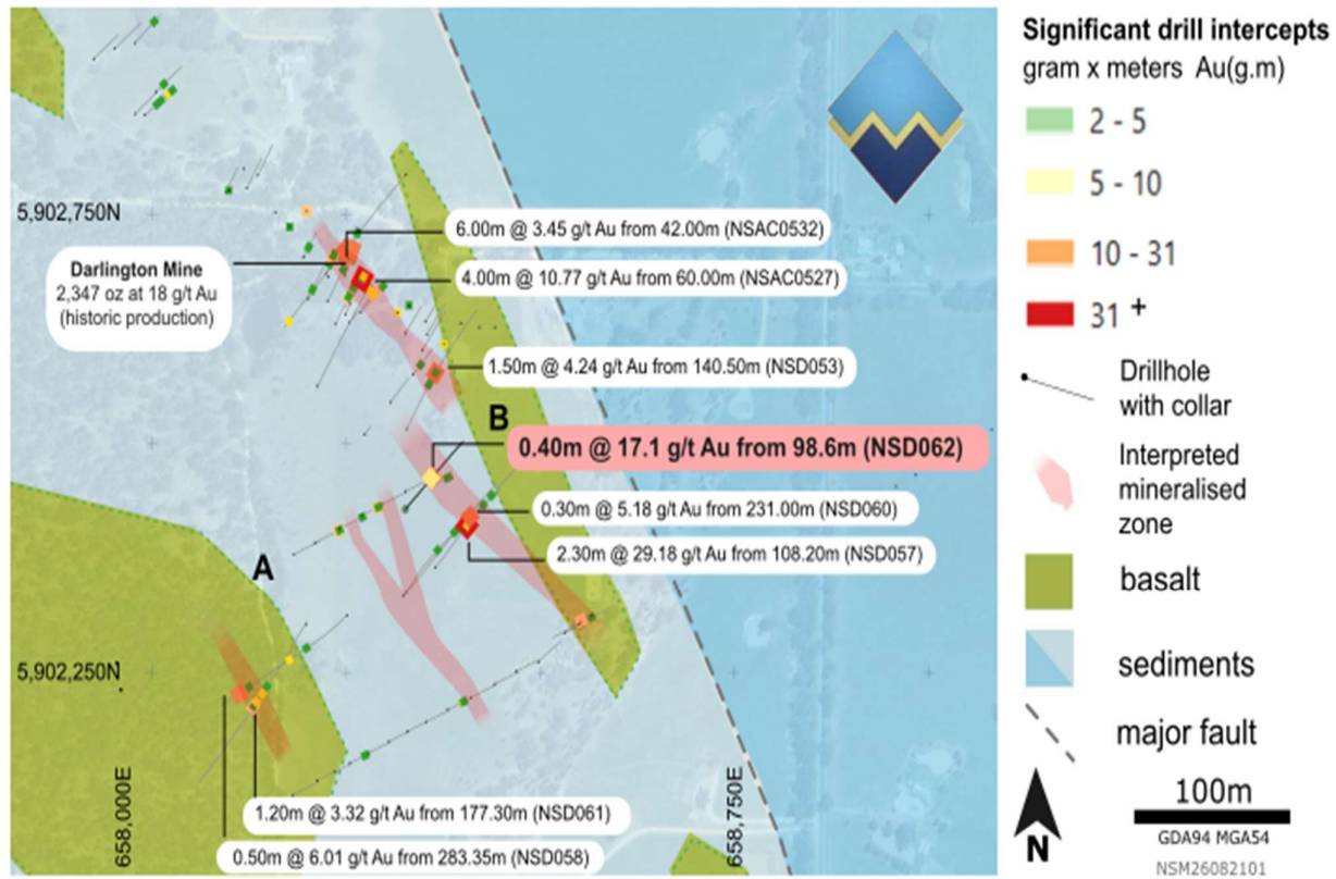
Figure 4 Plan view highlighting the strong continuity of the strike extension between NSD057 and NSD062.
