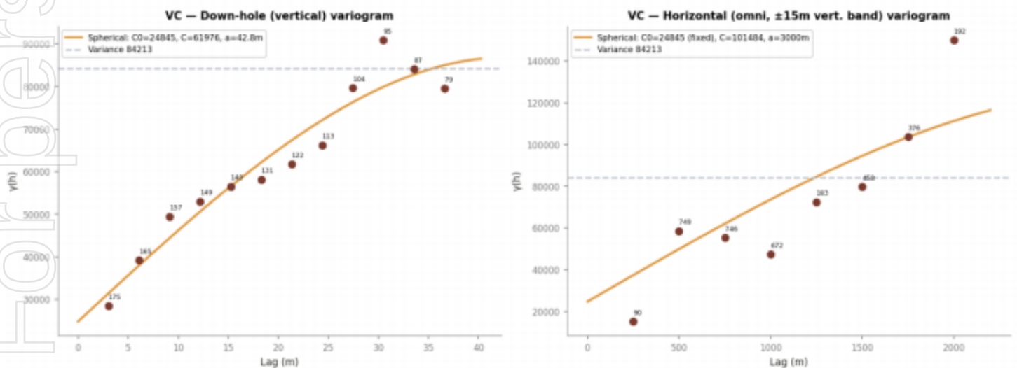
Figure 7: Experimental VC variograms and directional model fits used to assess continuity: downhole direction (left) and detrended horizontal direction (right).
