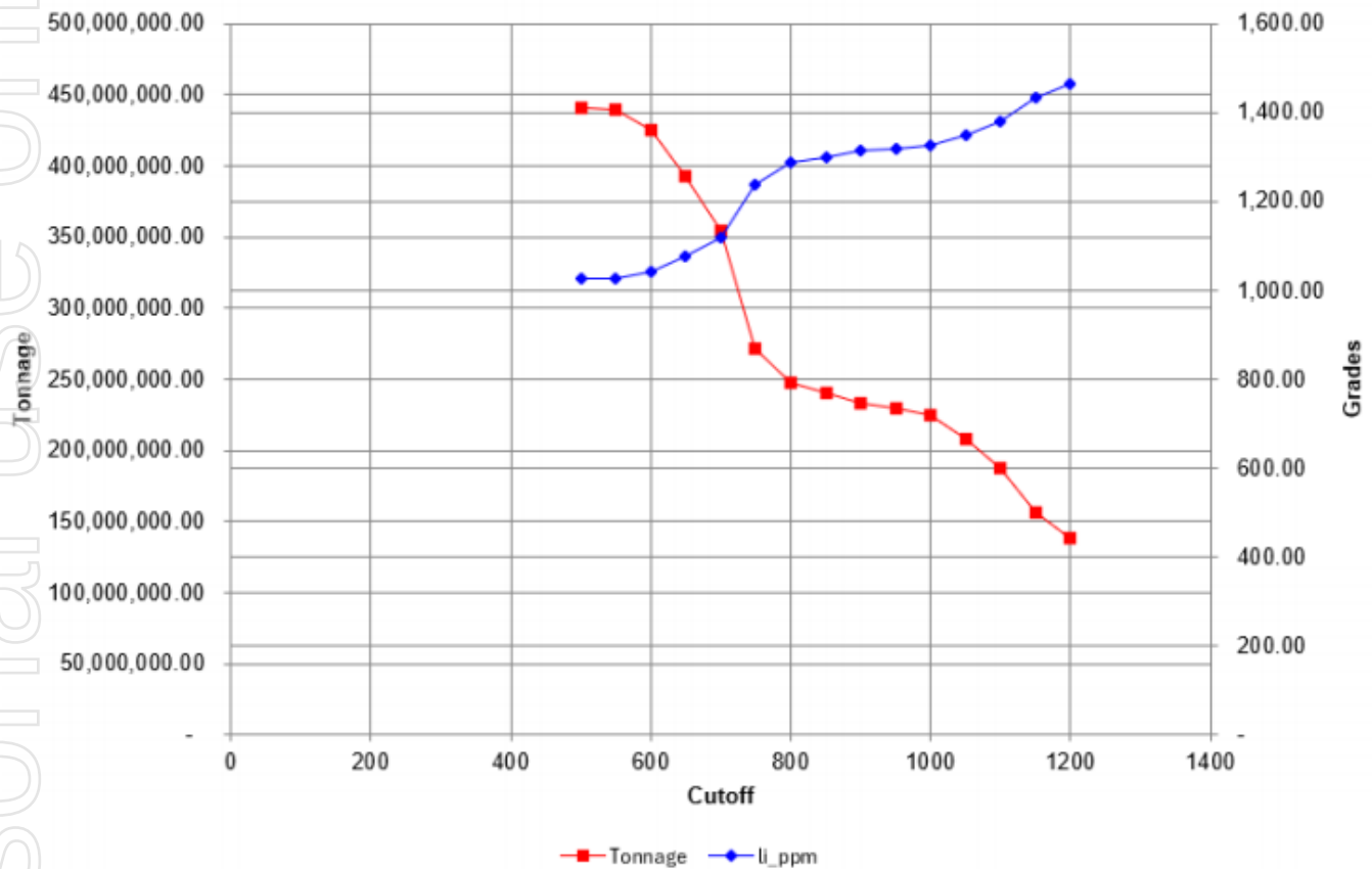
Figure 8: Grade-tonnage sensitivity for the conceptual VC Exploration Target in the northwestern extension. The results are based on extrapolated geometry and an adopted analogue bulk density and do not constitute a Mineral Resource. The curves illustrate sensitivity to cut-off grade and do not establish an economic cut-off.
