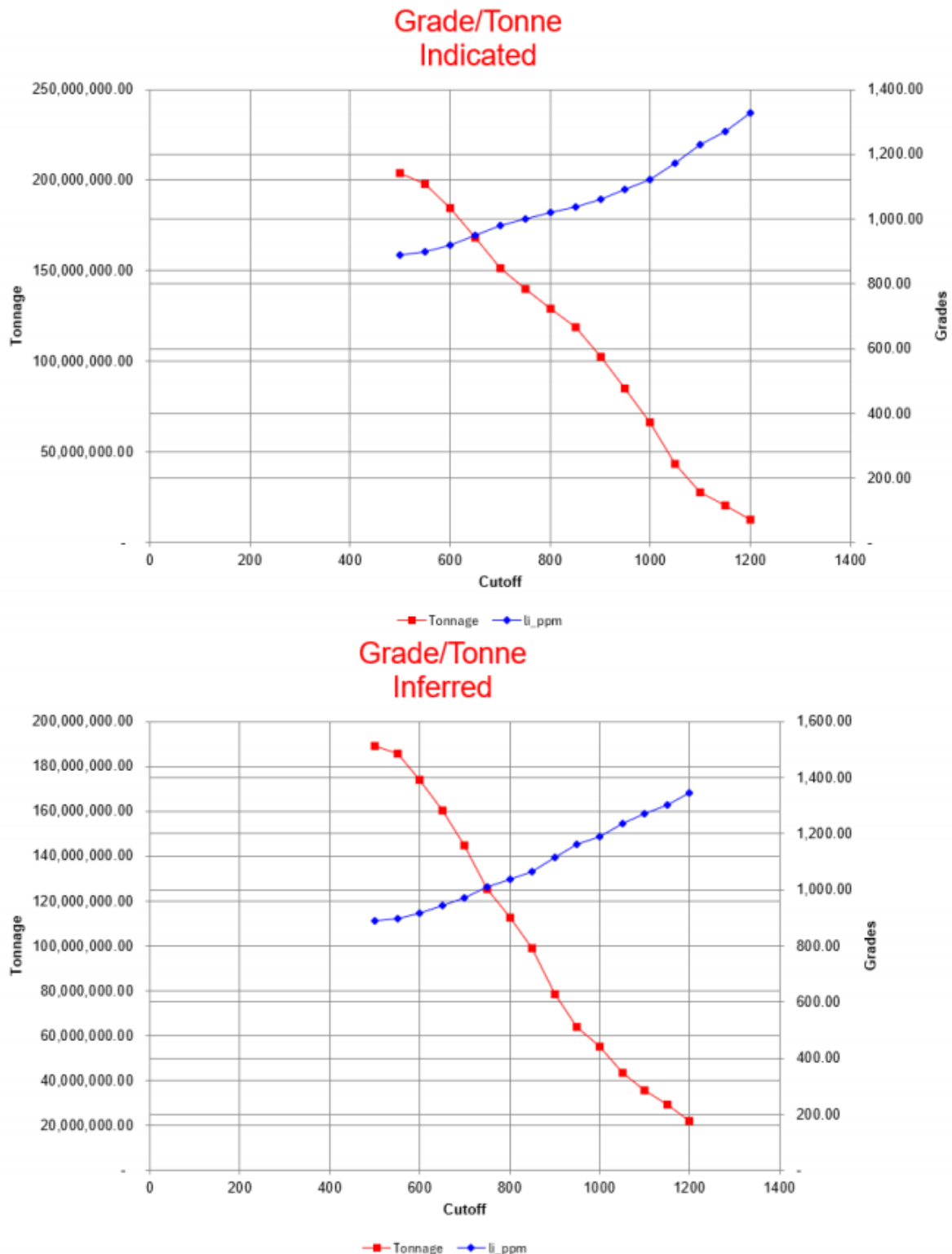
Figure 4: Grade-tonnage sensitivity for the Indicated (top) and Inferred (bottom) portions of the claim-constrained VC block model. The curves show changes in reported tonnage and average lithium grade with increasing cut-off grade and do not independently establish an economic cut-off.
