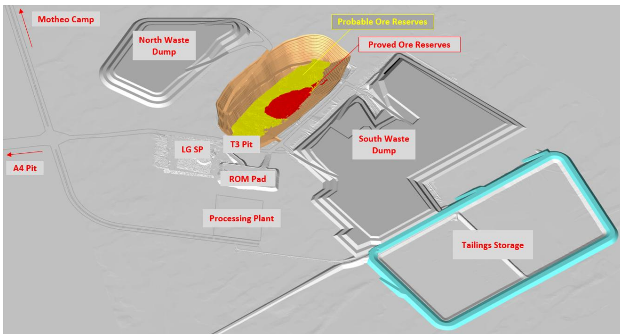
Figure 7: T3 Copper Project – Site Layout
