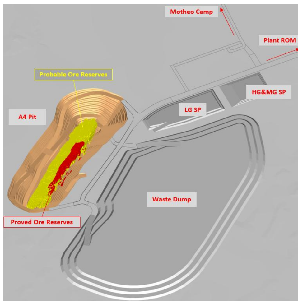
Figure 8: A4 Copper Project – Site Layout
