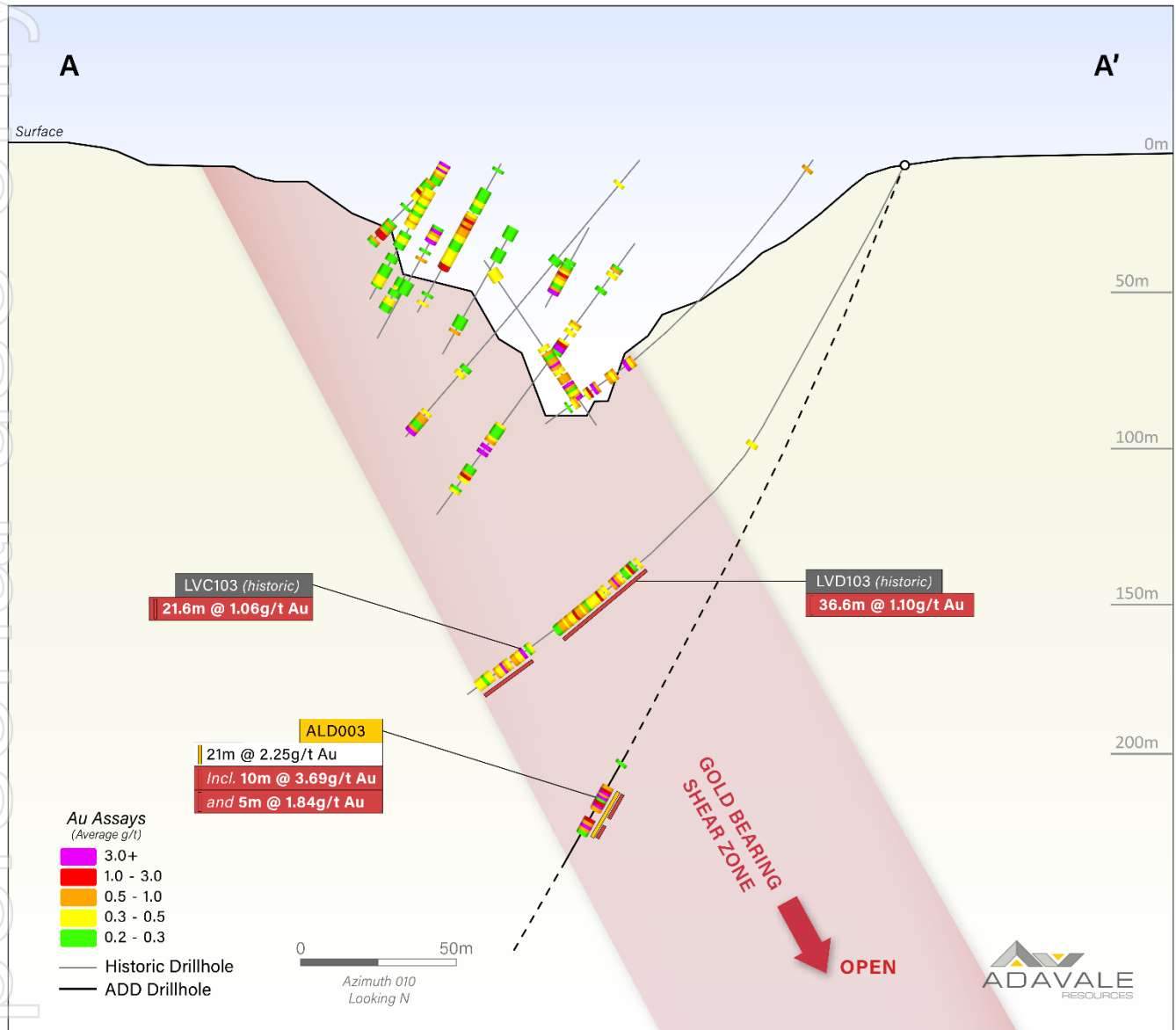
Figure 2: Cross Section showing position and gold results for ALD003 relative to the historic London-Victoria Open Pit (Section Line A-A' displayed in Figure 1)
