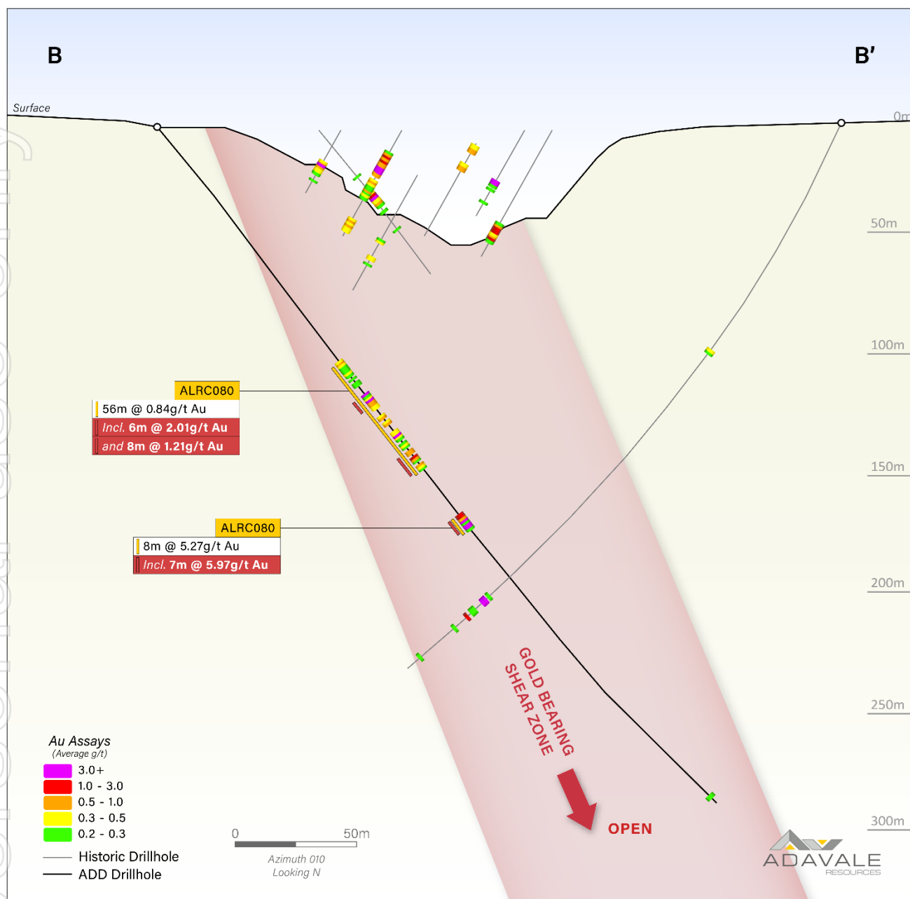
Figure 3: Cross Section showing position and gold results for ALRC080 relative to the historic London-Victoria Open Pit (Section Line B-B' displayed in Figure 1)
