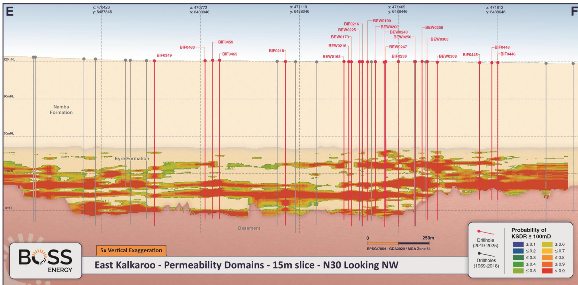
Figure 4: Cross-section view of East Kalkaroo, displaying the probability of KSDR values \geq 100 mD
