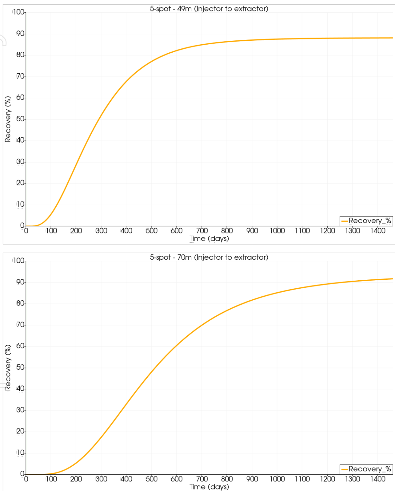
Figure 19: Example of RTM-simulated recovery curves for two alternative wellfield configurations. The 49 m injector-to-extractor spacing is shown above and the 70 m injector-to-extractor configuration is shown below. The recovery curves correspond to the same wellfields used to illustrate the two configurations in Figure 18.
