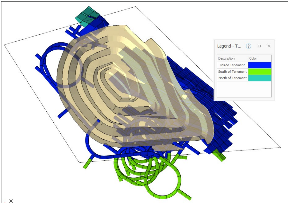
Figure 18 - LOM Mine Design Tenement Boundaries - Plan View
