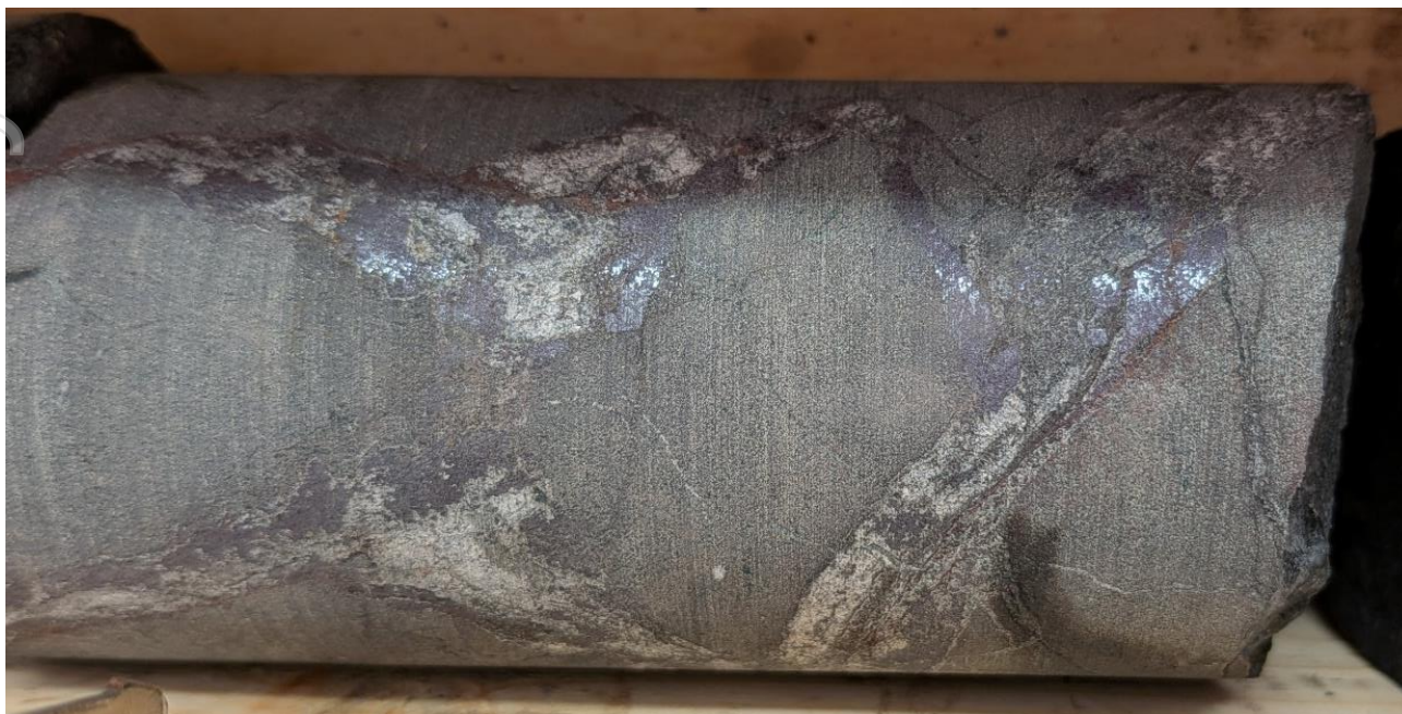
Figure 8 - Photograph of vein and breccia cement hosted chalcocite mineralisation that characterises the sulphides between 76m and 80m in DAN26047. Drill core is NQ2 diameter.
