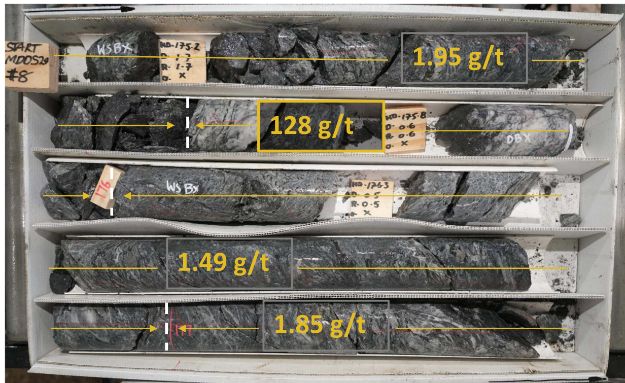
Figure 2. High-grade Au intervals in MDD529 sampled to geology
