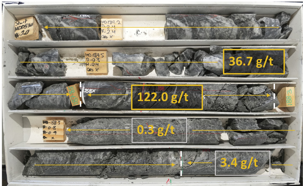
Figure 3. High-grade Au intervals in MDD530 sampled to geology
