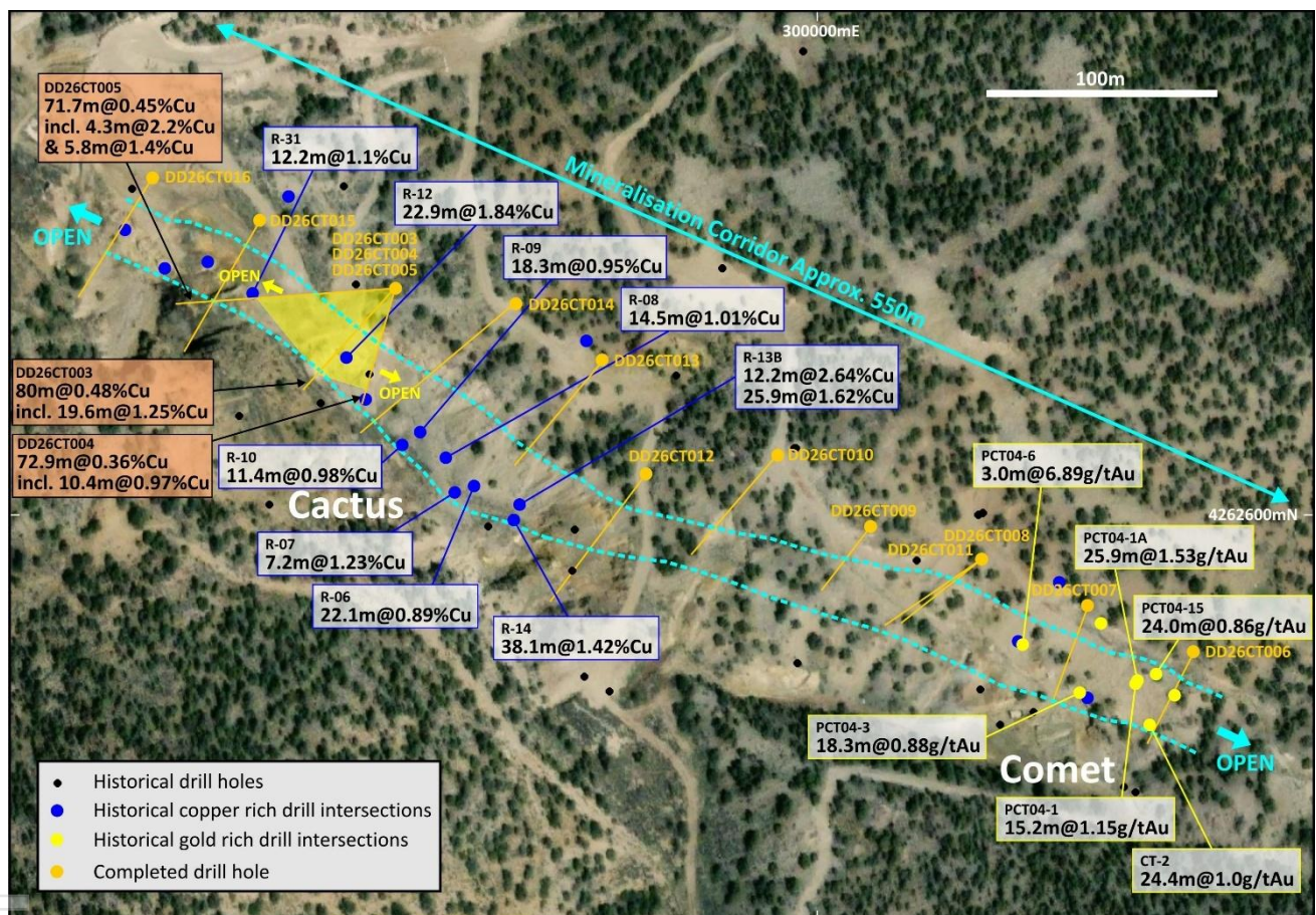
Figure 2: Location of all Hawk drill holes (DD26CT006-016) in the Comet and Cactus zones of the just completed Cactus Corridor drilling programme and historical shallow drill hole intersections.
